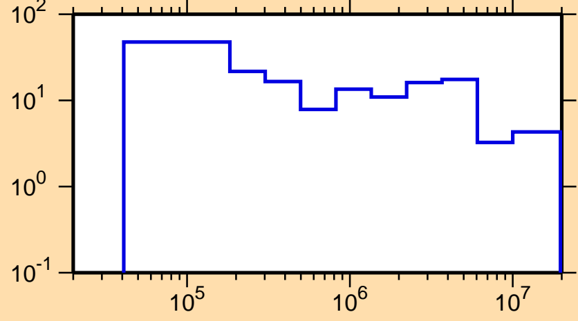
\Delta\sigma/\sigma vs. E for ^{181}\text{Hf}(n,\text{el.})
