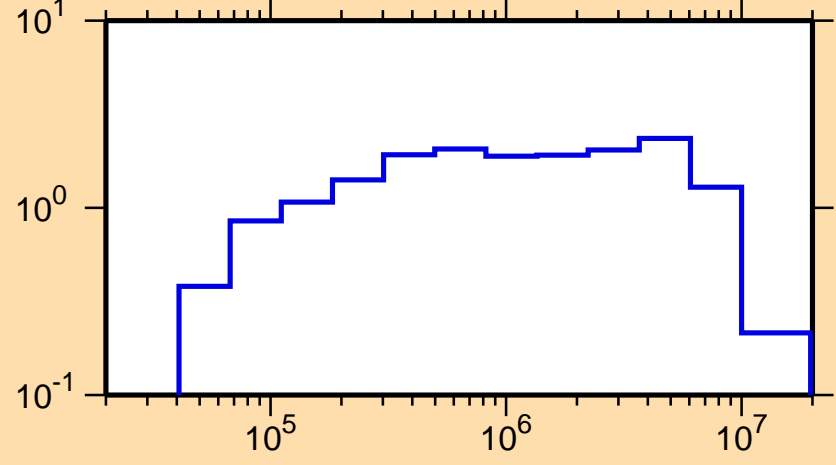
\sigma vs. E for ^{181}\text{Hf}(n,\text{inel.})
