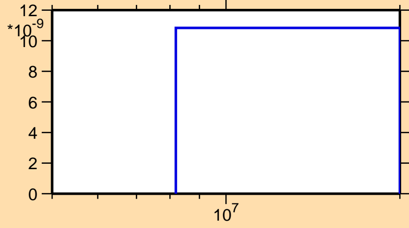
\sigma vs. E for ^{181}\text{Hf}(n,\text{nd})
