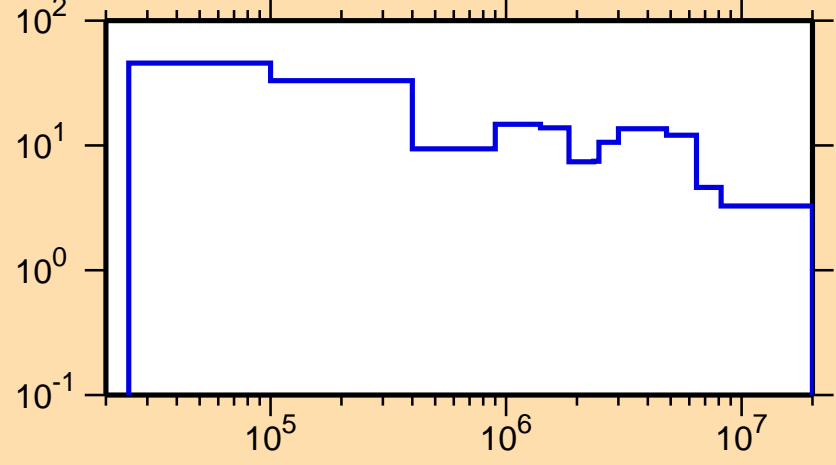
\Delta\sigma/\sigma vs. E for ^{181}\text{Hf}(n,\text{tot.})
