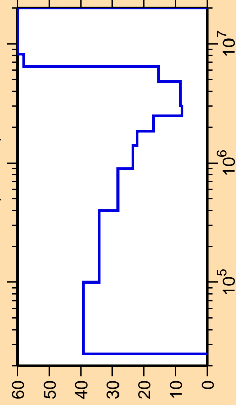
\Delta\sigma/\sigma vs. E for ^{181}\text{Hf}(n,\text{inel.})
