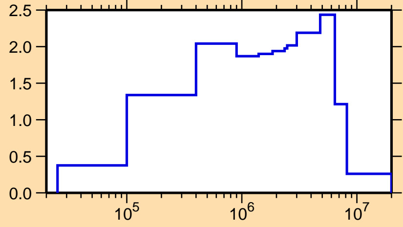
\sigma vs. E for ^{181}\text{Hf}(n,\text{inel.})
