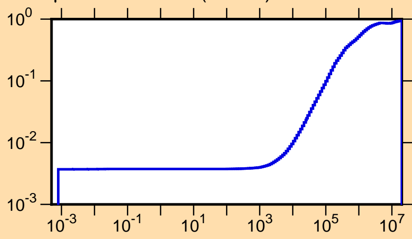
\mu vs. E for ^{182}\text{Hf}(\text{mt251})
