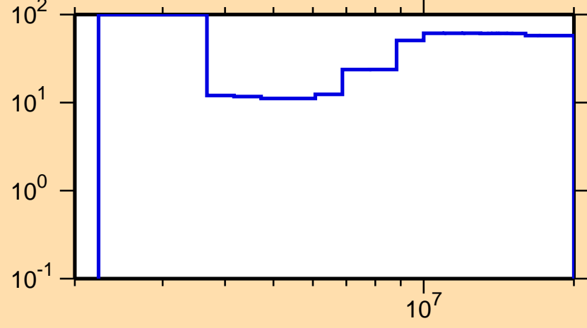
\Delta\sigma/\sigma vs. E for ^{182}\text{Hf}(n,n\text{cont.})
