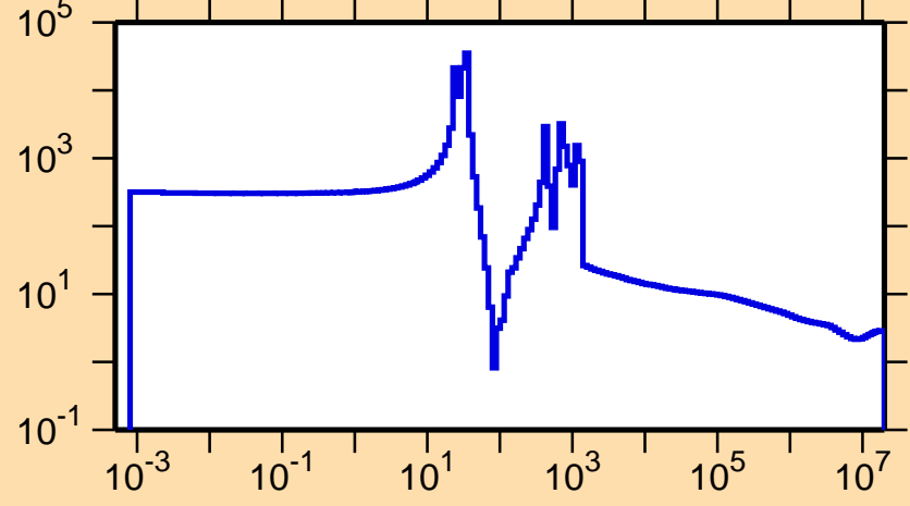
\sigma vs. E for ^{182}\text{Hf}(n,\text{el.})
