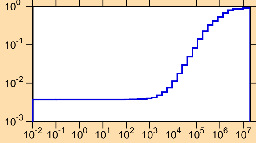
\mu vs. E for ^{182}\text{Hf}(\text{mt251})
