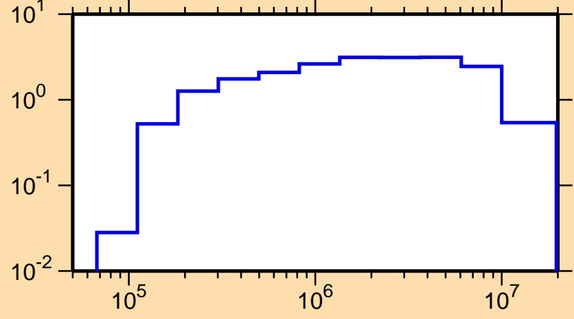
\sigma vs. E for ^{182}\text{Hf}(n,\text{inel.})
