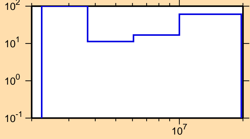
\Delta\sigma/\sigma vs. E for ^{182}\text{Hf}(n,ncont.)
