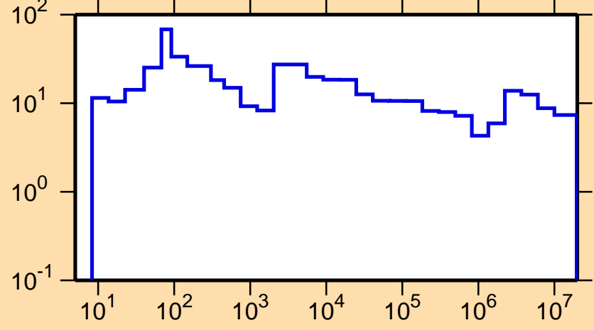
\Delta\sigma/\sigma vs. E for ^{182}\text{Hf}(n, \text{el.})
