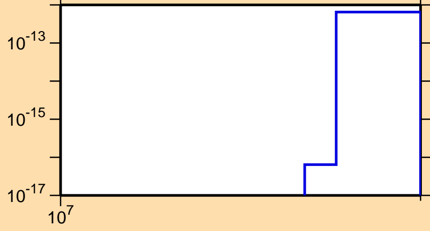
\sigma vs. E for ^{183}\text{Hf}(n,3n\alpha)
