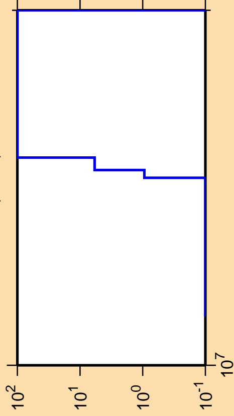
\Delta\sigma/\sigma vs. E for ^{183}\text{Hf}(n,nd)
