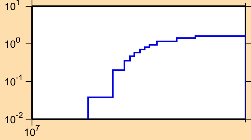
\sigma vs. E for ^{183}\text{Hf}(n,3n)
