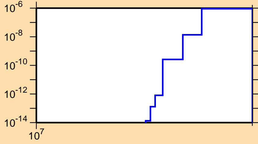
\sigma vs. E for ^{183}\text{Hf}(n,nd)
