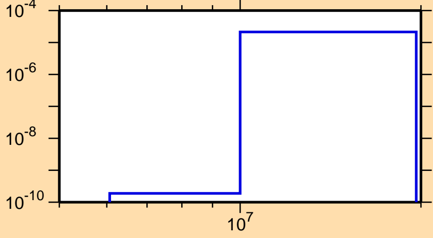
\sigma vs. E for ^{183}\text{Hf}(n,\alpha)
