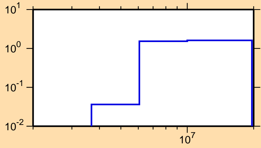
\sigma vs. E for ^{183}\text{Hf}(n,2n)
