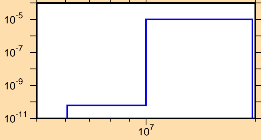
\sigma vs. E for ^{184}\text{Hf}(n,\alpha)
