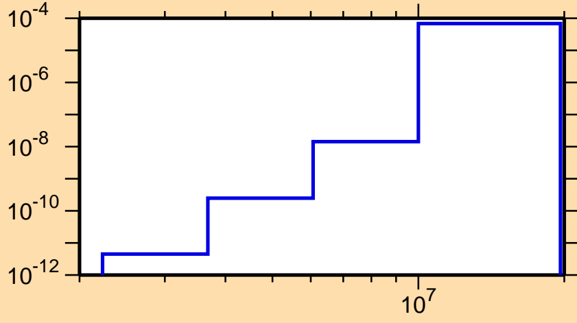
\sigma vs. E for ^{184}\text{Hf}(n,\alpha)
