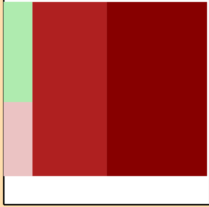
\Delta\sigma/\sigma vs. E for ^{184}\text{Hf}(n,\text{el.})
