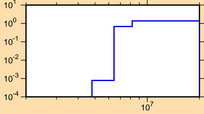
\sigma vs. E for ^{184}\text{Hf}(n,2n)
