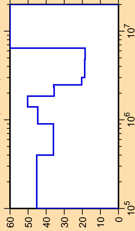
\Delta\sigma/\sigma vs. E for ^{184}\text{Hf}(n,\text{inel.})
