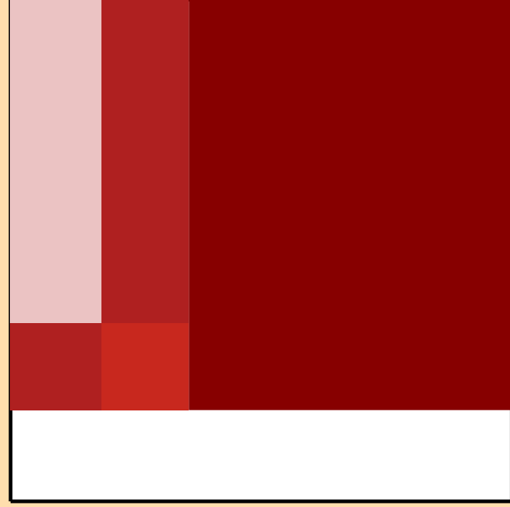
\Delta\sigma/\sigma vs. E for ^{184}\text{Hf}(n,el.)
