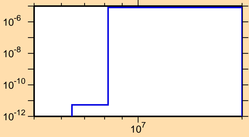
\sigma vs. E for ^{184}\text{Hf}(n,\alpha)
