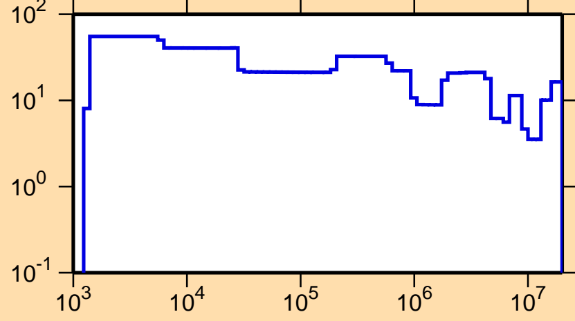
\Delta\sigma/\sigma vs. E for ^{184}\text{Hf}(n,\text{tot.})
