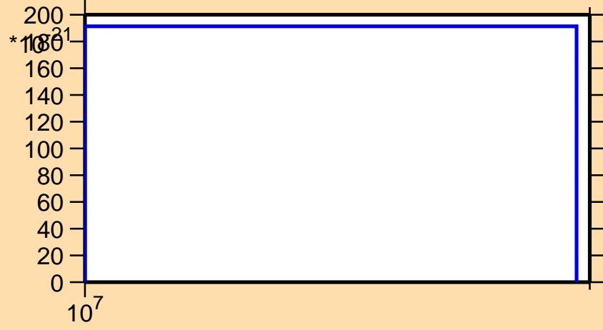
\sigma vs. E for ^{184}\text{Hf} (mt 42)
