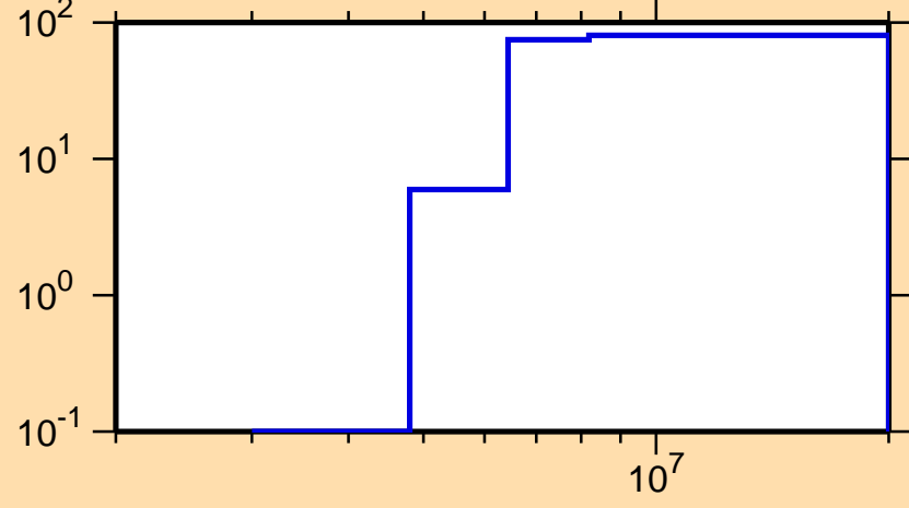
\Delta\sigma/\sigma vs. E for ^{184}\text{Hf}(n,p)
