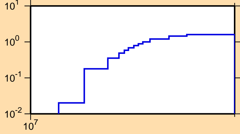
\sigma vs. E for ^{185}\text{Hf}(n,3n)
