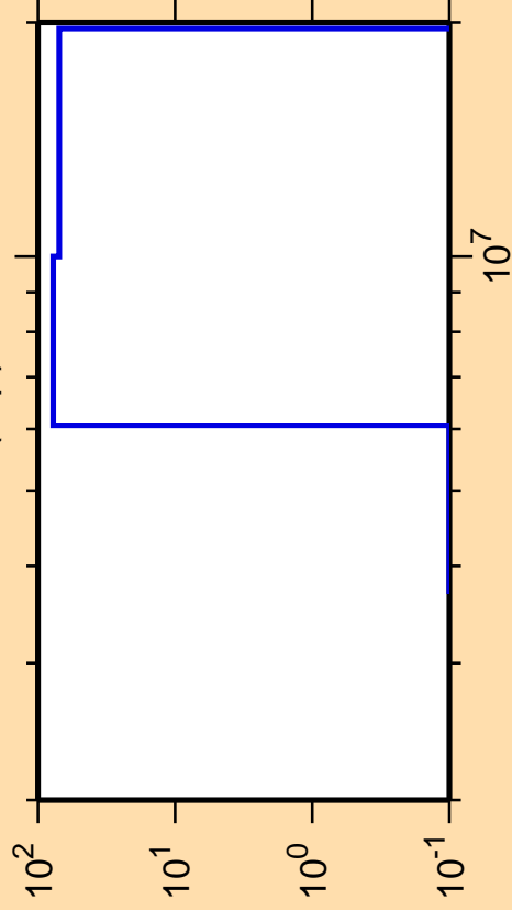
\Delta\sigma/\sigma vs. E for ^{185}\text{Hf}(n,p)
