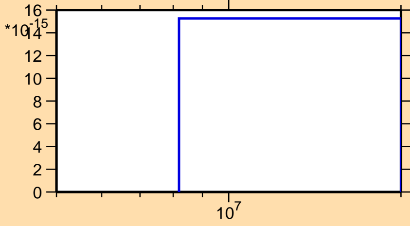
\sigma vs. E for ^{185}\text{Hf}(n,3n\alpha)
