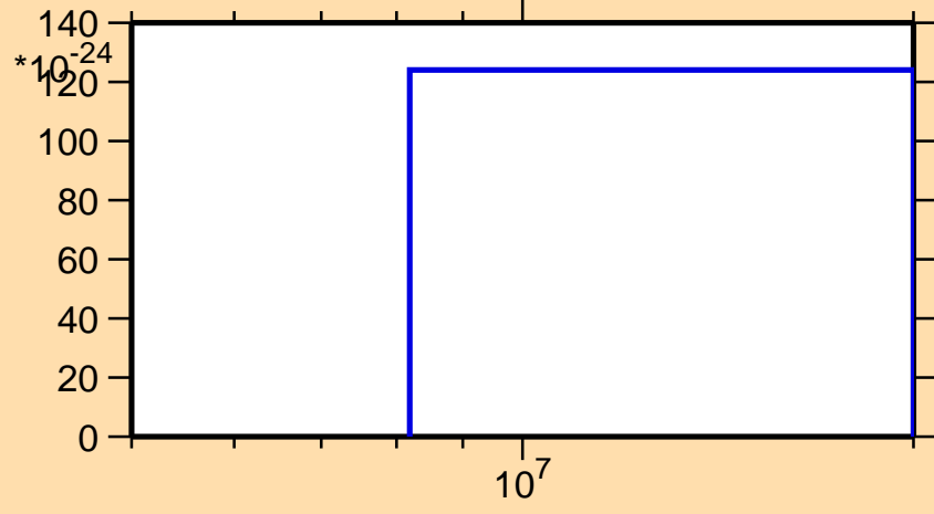
\sigma vs. E for ^{185}\text{Hf} (mt 42)
