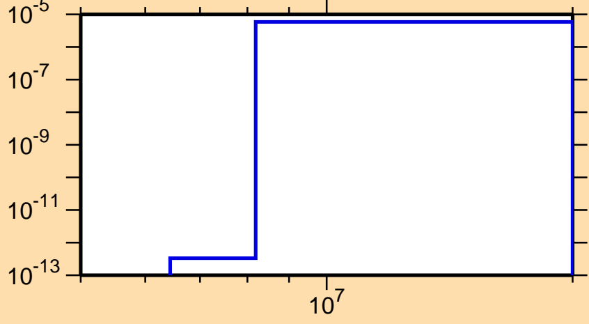
\sigma vs. E for ^{185}\text{Hf}(n,n\alpha)
