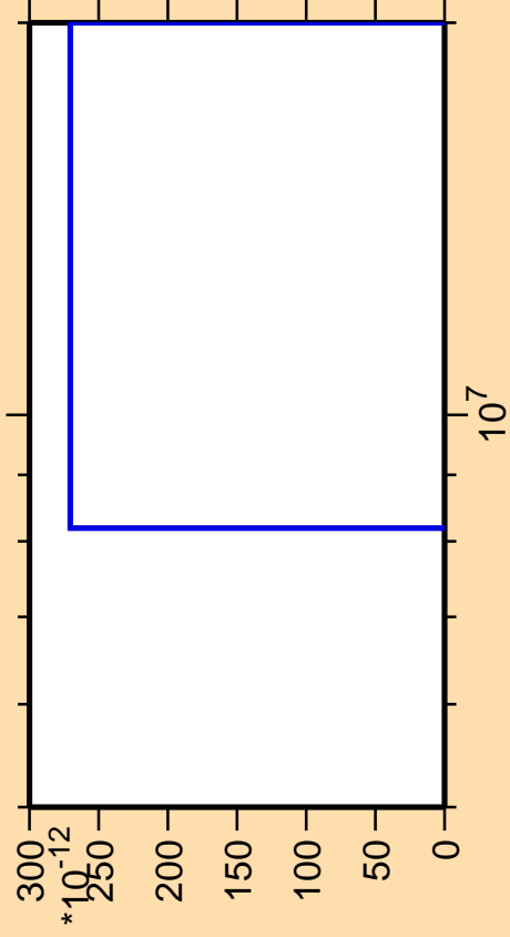
\Delta\sigma/\sigma vs. E for ^{185}\text{Hf} (mt 42)
