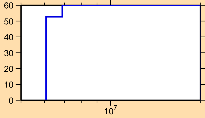
\Delta\sigma/\sigma vs. E for ^{186}\text{Hf}(n,ncont.)
