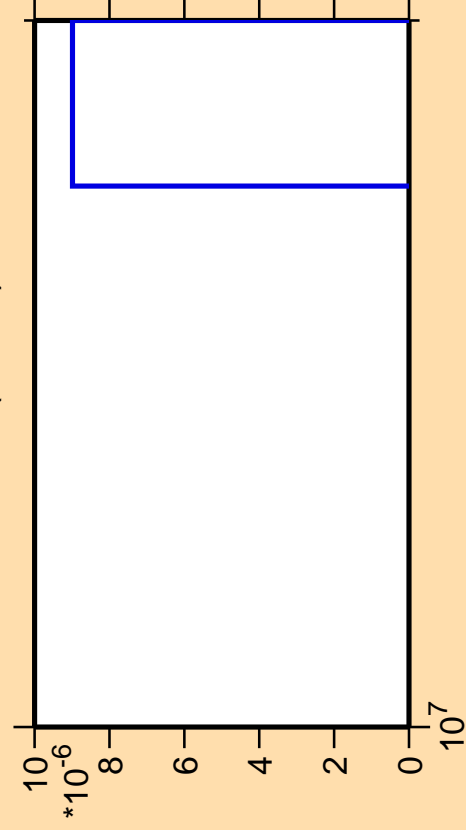
\Delta\sigma/\sigma vs. E for ^{186}\text{Hf} (mt 11)
