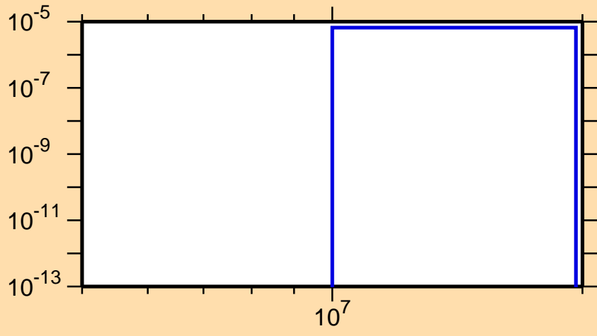
\sigma vs. E for ^{186}\text{Hf}(n,d)
