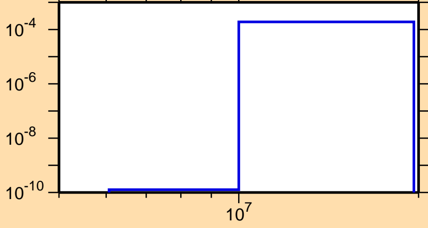
\sigma vs. E for ^{186}\text{Hf}(n,p)
