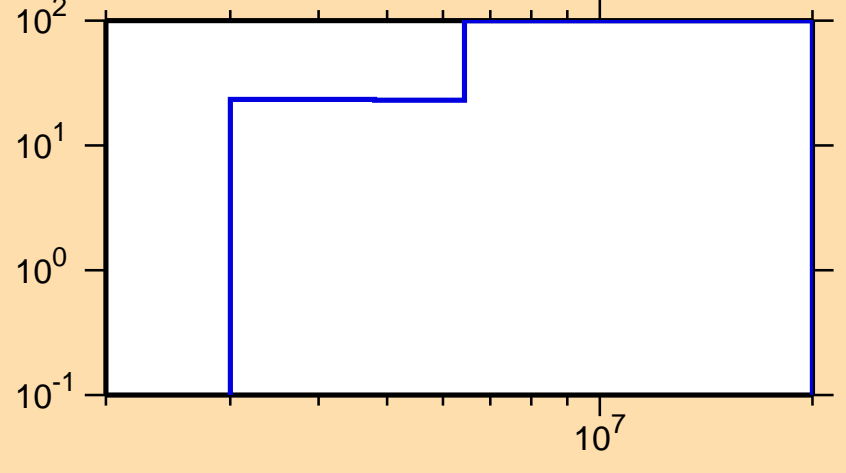
\Delta\sigma/\sigma vs. E for ^{186}\text{Hf}(n,n\text{cont.})
