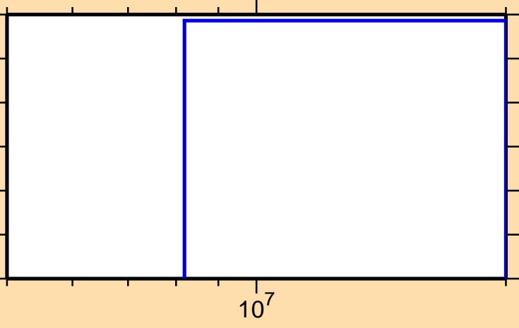
\sigma vs. E for ^{186}\text{Hf}(n,t)
