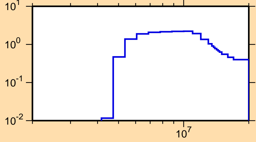
\sigma vs. E for ^{187}\text{Hf}(n,2n)
