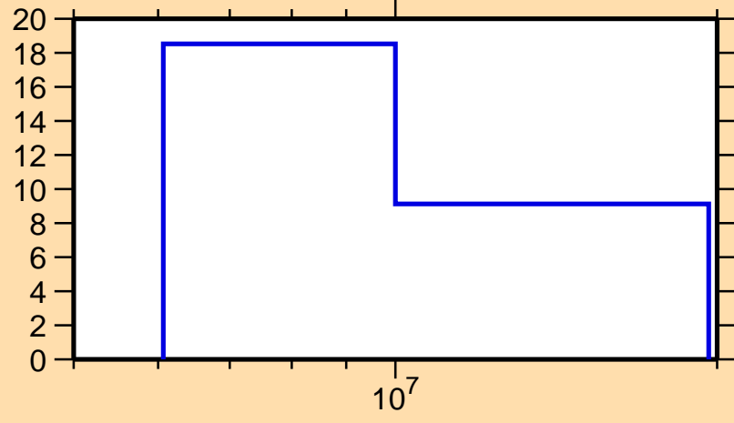
\Delta\sigma/\sigma vs. E for ^{187}\text{Hf}(n,el.)
