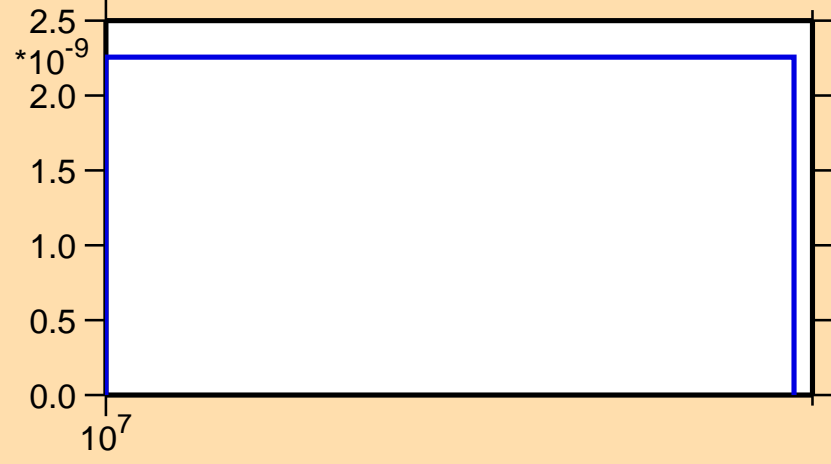
\sigma vs. E for ^{187}\text{Hf}(n,\text{nd})
