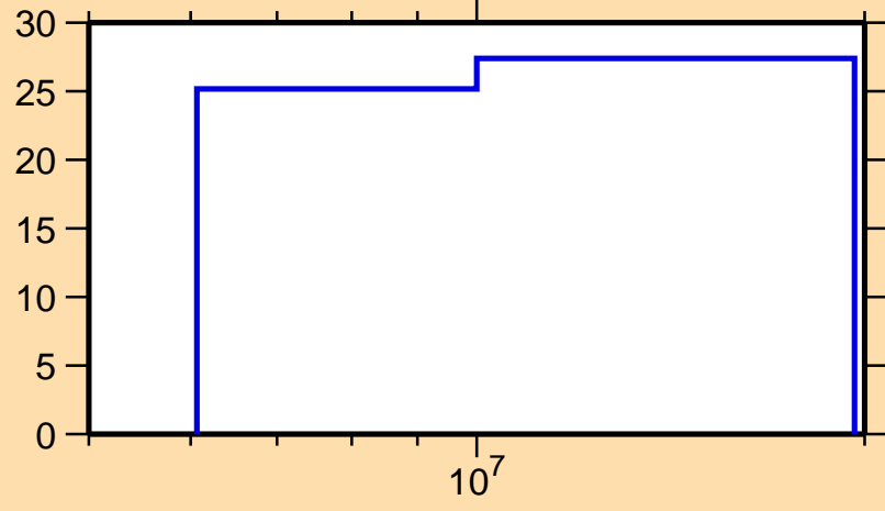
\Delta\sigma/\sigma vs. E for ^{187}\text{Hf}(n,2n)
