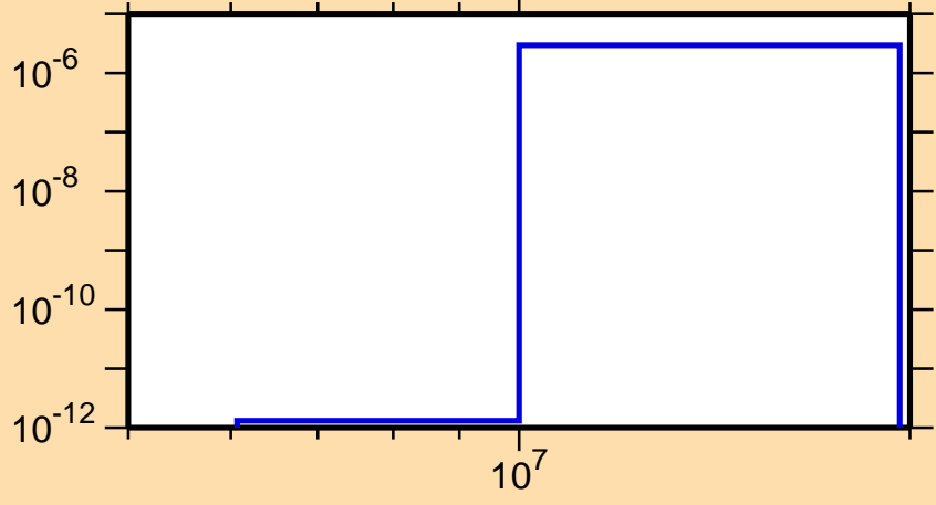
\sigma vs. E for ^{187}\text{Hf}(n,\alpha)
