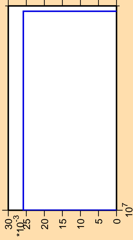
\Delta\sigma/\sigma vs. E for ^{187}\text{Hf}(n,3n\alpha)
