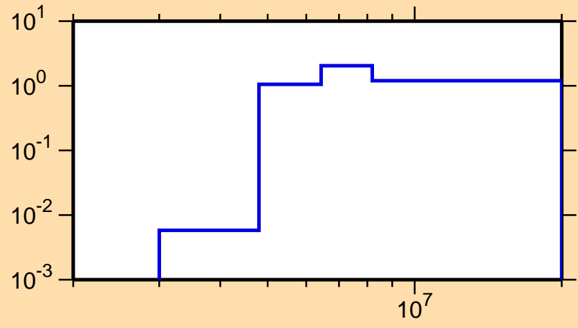
\sigma vs. E for ^{187}\text{Hf}(n,2n)
