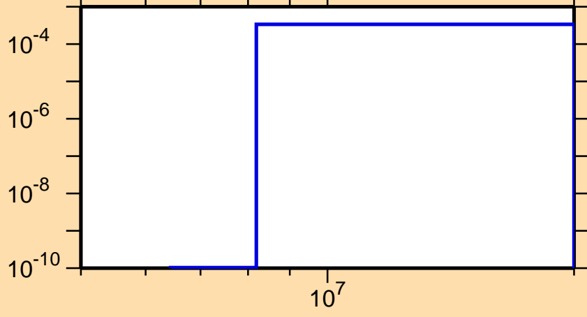
\sigma vs. E for ^{187}\text{Hf}(n,p)
