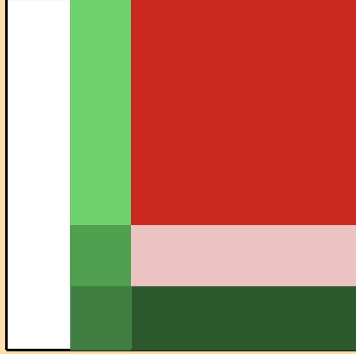
\Delta\sigma/\sigma vs. E for ^{187}\text{Hf}(n,p)
