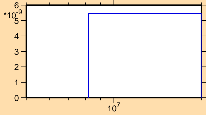
\sigma vs. E for ^{187}\text{Hf}(n,nt)
