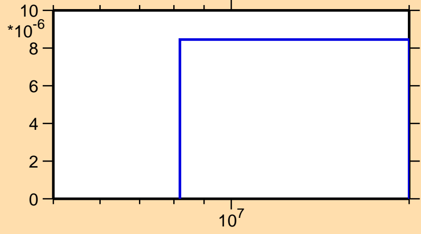
\sigma vs. E for ^{187}\text{Hf}(n,t)
