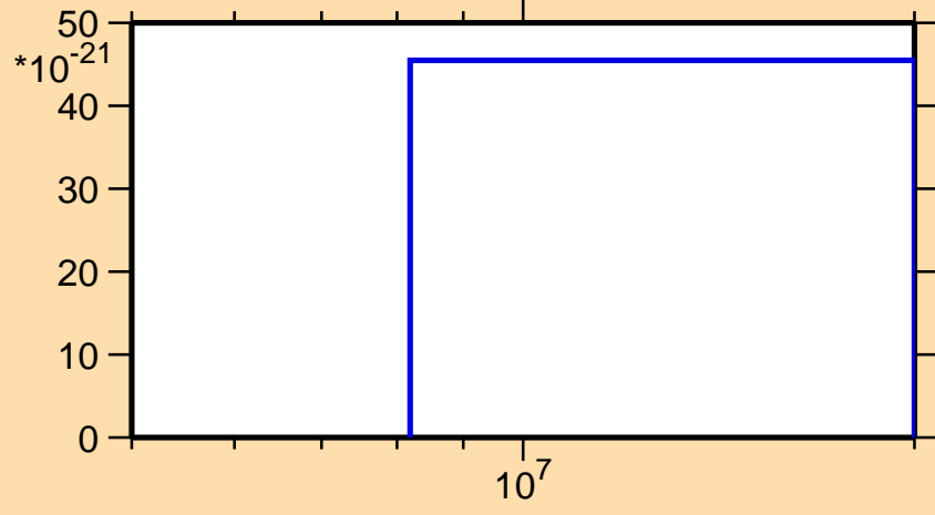
\sigma vs. E for ^{187}\text{Hf}(\text{mt } 42)
