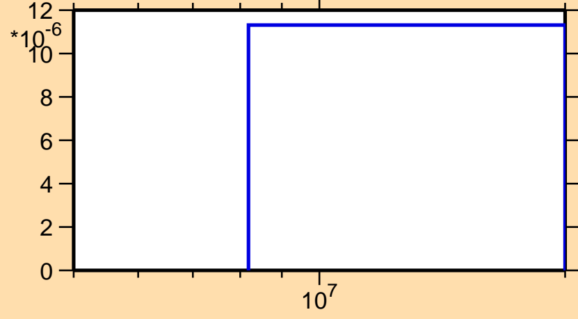
\sigma vs. E for ^{187}\text{Hf}(n,d)
