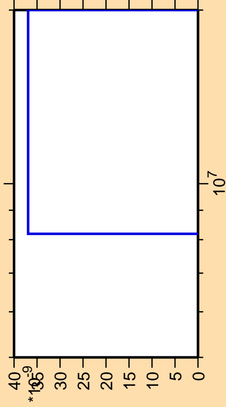
\Delta\sigma/\sigma vs. E for ^{187}\text{Hf}(\text{mt } 42)
