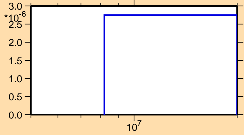
\sigma vs. E for ^{187}\text{Hf}(n,np)
