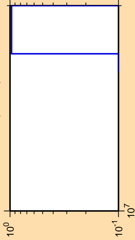
\Delta\sigma/\sigma vs. E for ^{188}\text{Hf}(n,3n\alpha)
