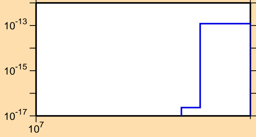
\sigma vs. E for ^{188}\text{Hf}(n,3n\alpha)
