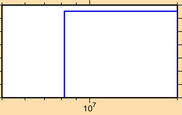
\sigma vs. E for ^{188}\text{Hf}(n,\alpha)
