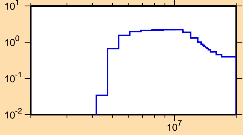
\sigma vs. E for ^{189}\text{Hf}(n,2n)
