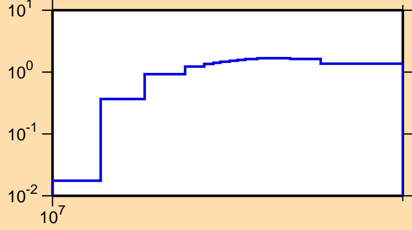
\sigma vs. E for ^{189}\text{Hf}(n,3n)
