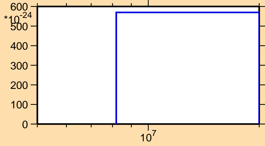
\sigma vs. E for ^{189}\text{Hf}(\text{mt } 11)
