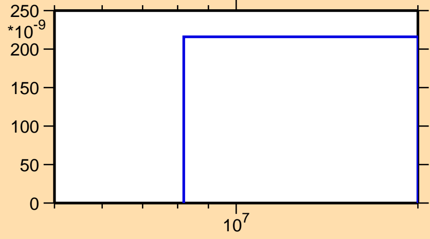
\sigma vs. E for ^{189}\text{Hf}(n,\alpha)
