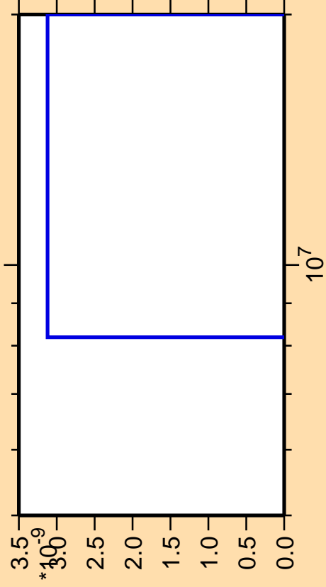
\Delta\sigma/\sigma vs. E for ^{189}\text{Hf}(\text{mt } 11)
