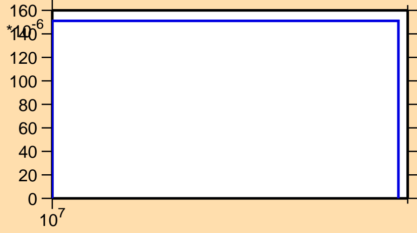
\sigma vs. E for ^{179}\text{Hg}(n,2np)
