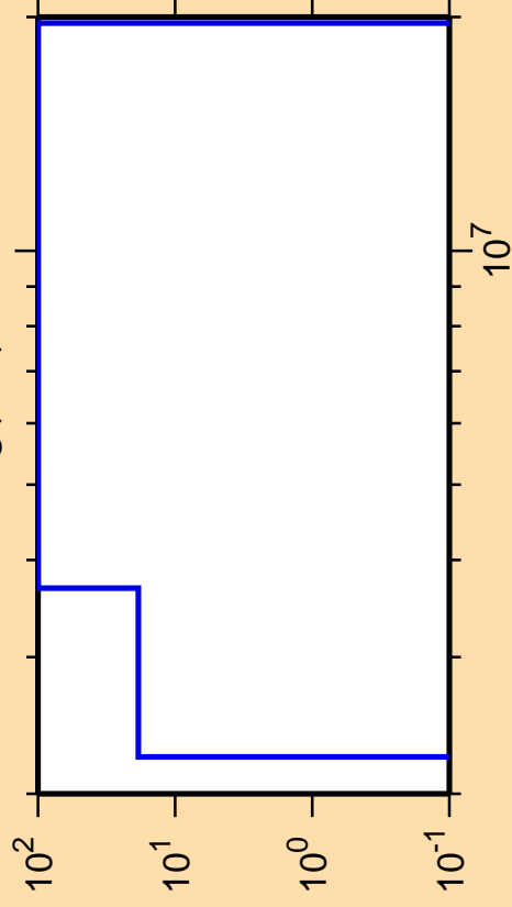
\Delta\sigma/\sigma vs. E for ^{179}\text{Hg}(n,d)
