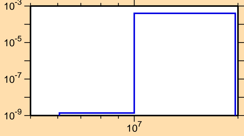
\sigma vs. E for ^{179}\text{Hg}(n,t)
