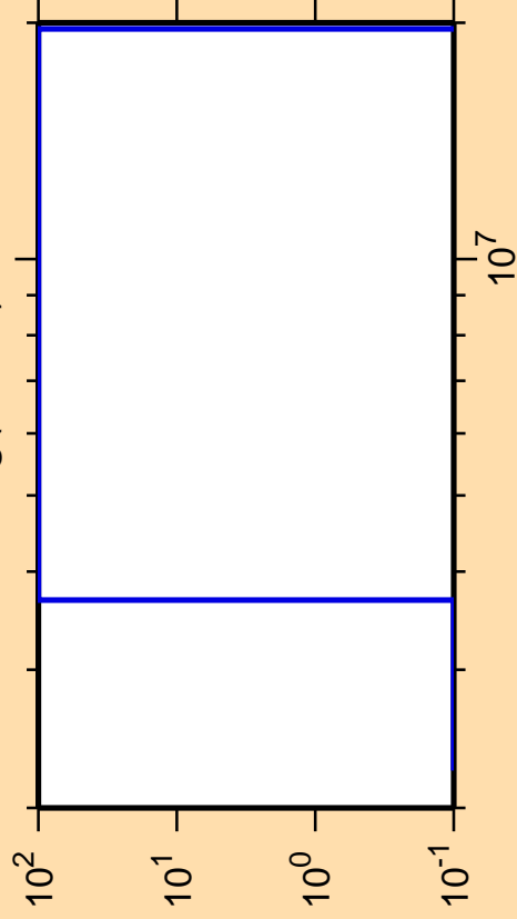
\Delta\sigma/\sigma vs. E for ^{179}\text{Hg} (mt 45)
