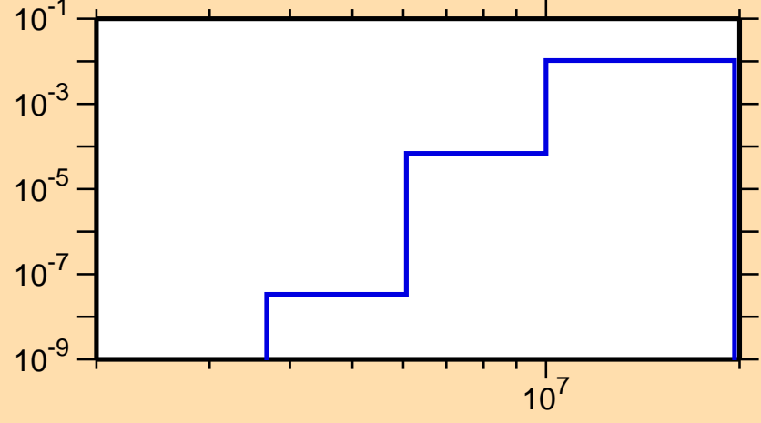
\sigma vs. E for ^{179}\text{Hg}(n,d)
