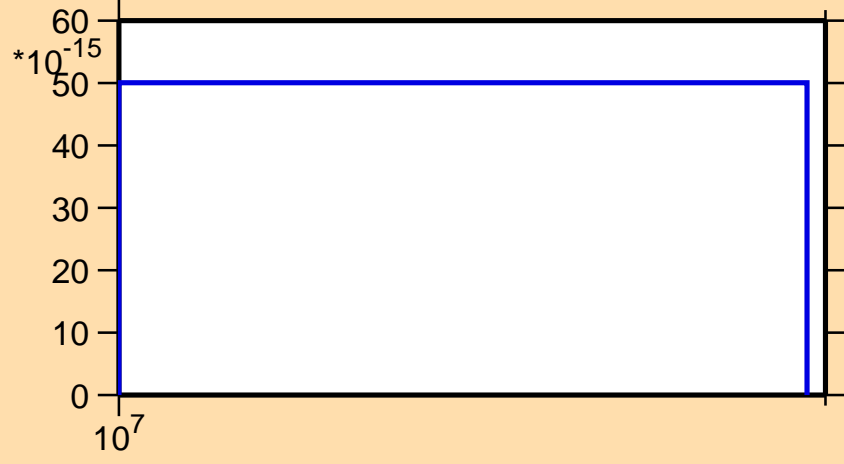
\sigma vs. E for ^{179}\text{Hg}(n,\text{nt})
