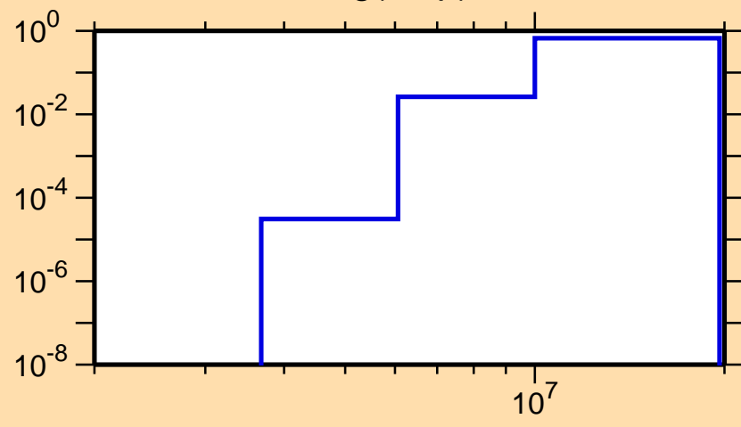
\sigma vs. E for ^{179}\text{Hg}(n,np)
