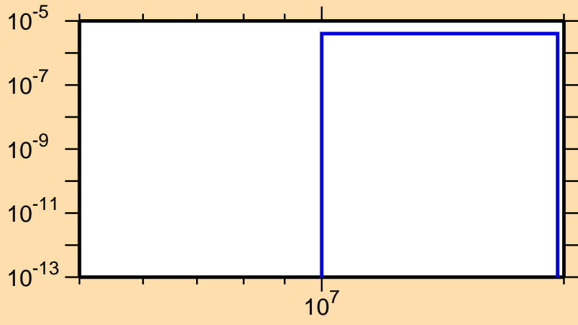
\sigma vs. E for ^{179}\text{Hg}(n,\text{pt})
