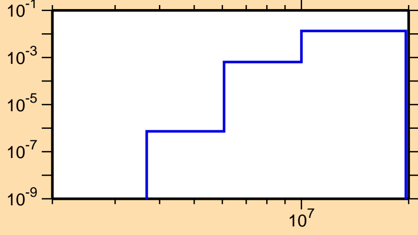
\sigma vs. E for ^{179}\text{Hg} (mt 45)
