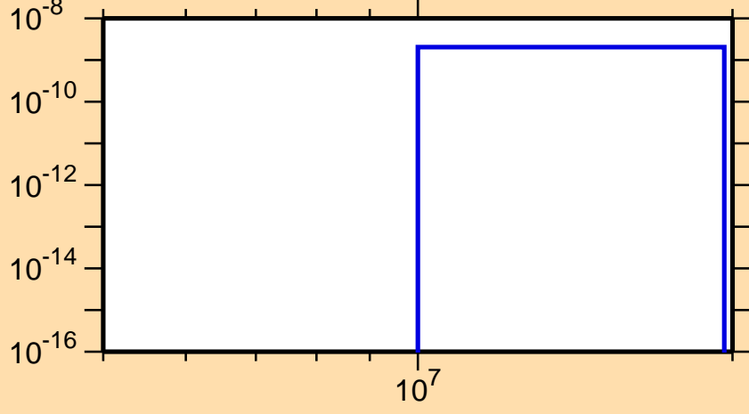
\sigma vs. E for ^{179}\text{Hg} (mt 34)
