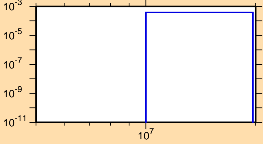
\sigma vs. E for ^{179}\text{Hg}(n,2n\alpha)
