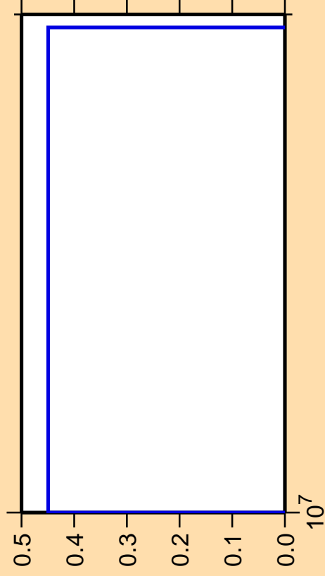
\Delta\sigma/\sigma vs. E for ^{179}\text{Hg}(n,\text{nt})
