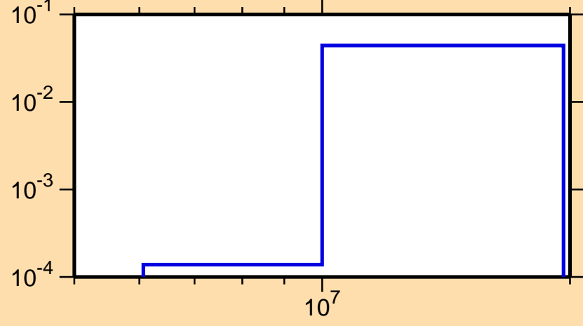
\sigma vs. E for ^{179}\text{Hg}(n,2n)
