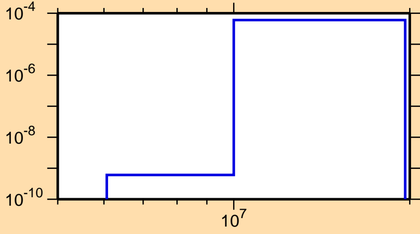
\sigma vs. E for ^{179}\text{Hg}(n,\text{pd})
