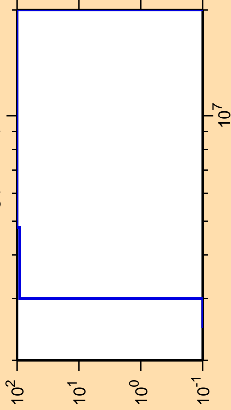
\Delta\sigma/\sigma vs. E for ^{179}\text{Hg}(\text{mt117})
