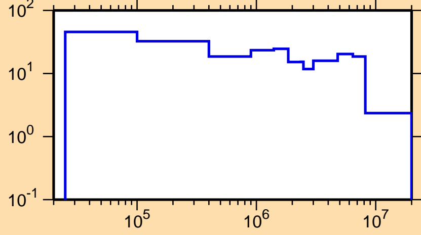
\Delta\sigma/\sigma vs. E for ^{179}\text{Hg}(n,\text{el.})
