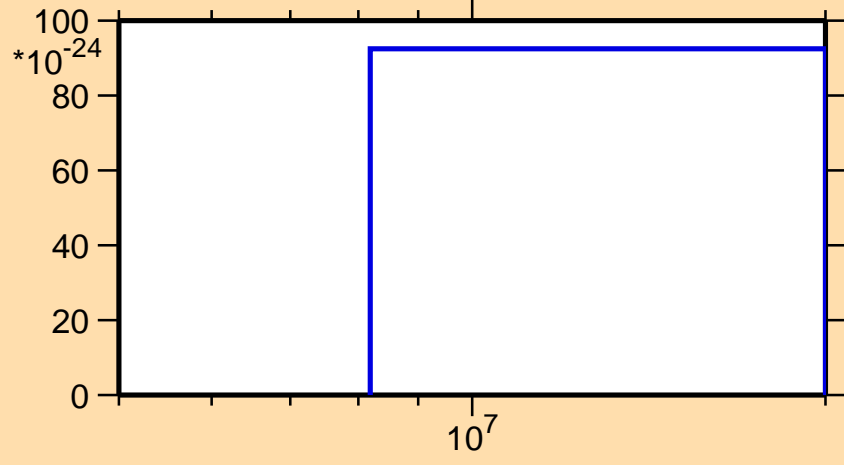
\sigma vs. E for ^{179}\text{Hg} (mt 11)
