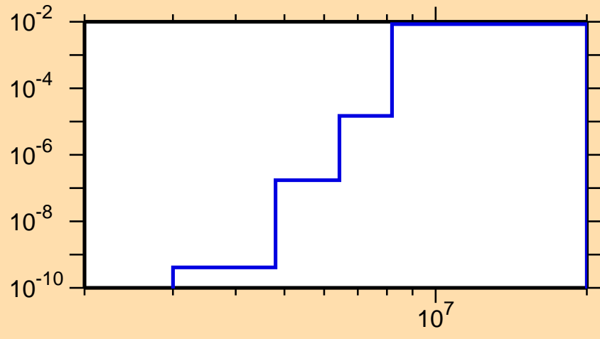
\sigma vs. E for ^{179}\text{Hg}(n,d)
