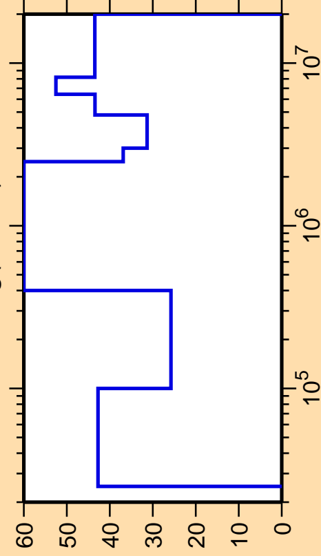
\Delta\sigma/\sigma vs. E for ^{179}\text{Hg}(n,\text{inel.})
