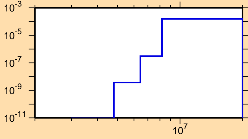
\sigma vs. E for ^{179}\text{Hg}(\text{mt117})
