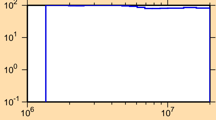
\Delta\sigma/\sigma vs. E for ^{180}\text{Hg}(n,ncont.)
