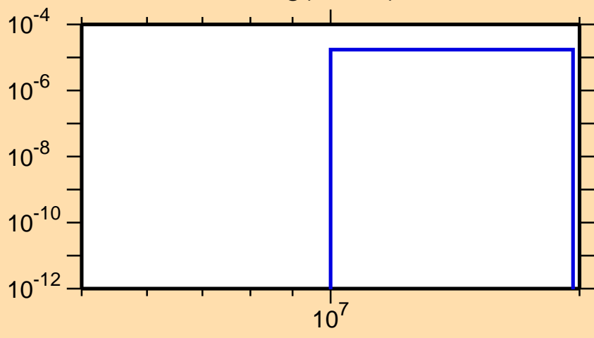
\sigma vs. E for ^{180}\text{Hg}(n,2n\alpha)
