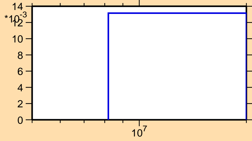
\sigma vs. E for ^{180}\text{Hg}(n,2n)
