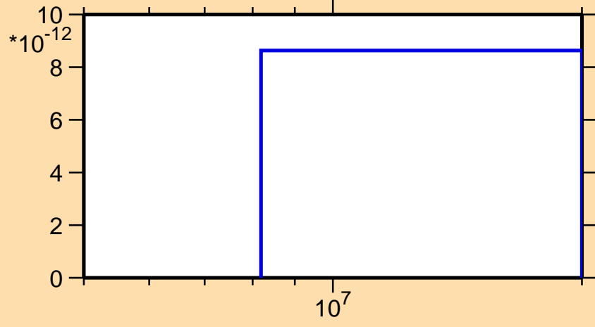
\sigma vs. E for ^{180}\text{Hg} (mt 34)
