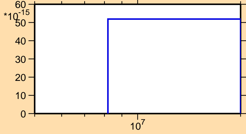
\sigma vs. E for ^{180}\text{Hg}(n,nt)
