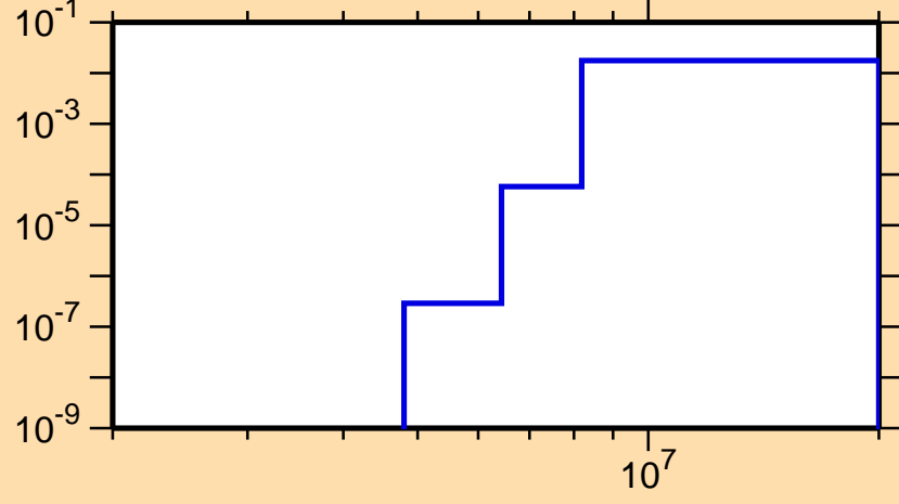
\sigma vs. E for ^{180}\text{Hg} (mt 45)
