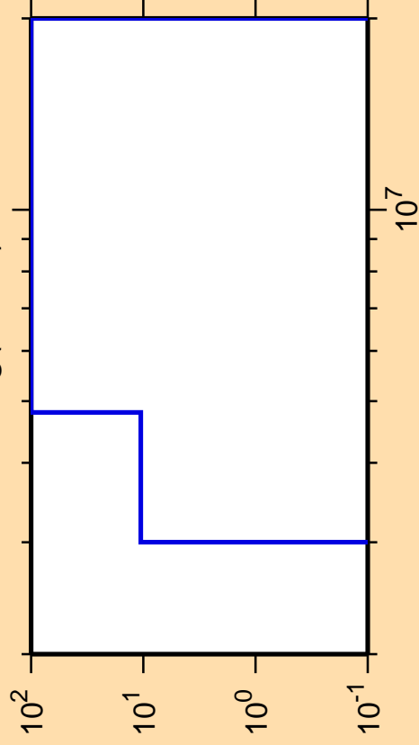
\Delta\sigma/\sigma vs. E for ^{180}\text{Hg} (mt 45)
