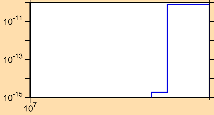
\sigma vs. E for ^{183}\text{Hg}(n,nt)
