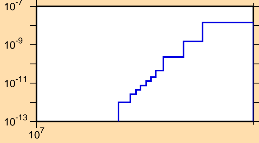
\sigma vs. E for ^{183}\text{Hg} (mt 34)
