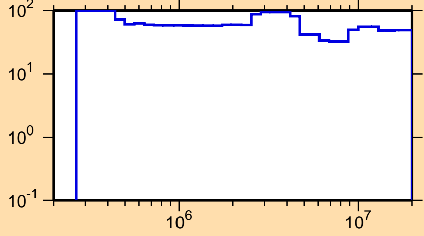
\Delta\sigma/\sigma vs. E for ^{183}\text{Hg}(n,ncont.)
