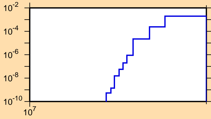
\sigma vs. E for ^{183}\text{Hg}(n,2np)
