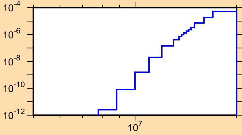
\sigma vs. E for ^{183}\text{Hg} (mt 45)
