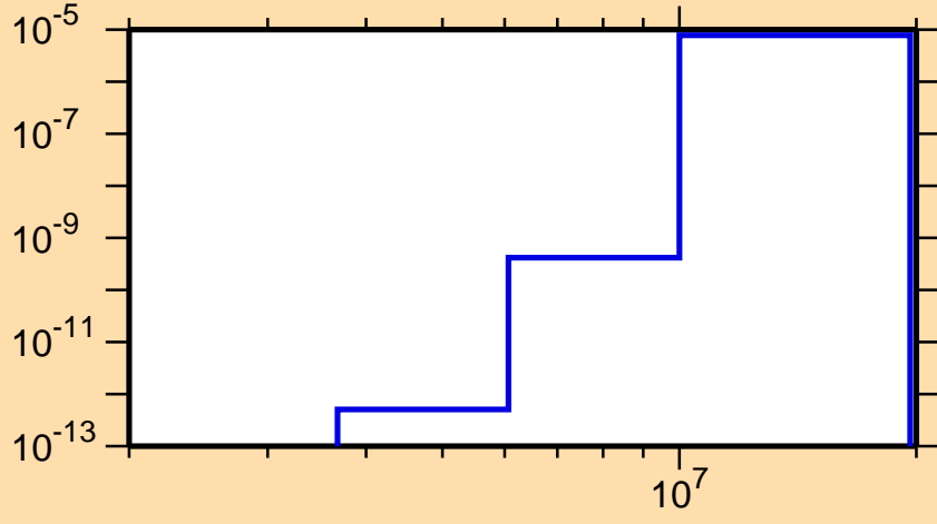
\sigma vs. E for ^{183}\text{Hg}(n,\text{He}3)
