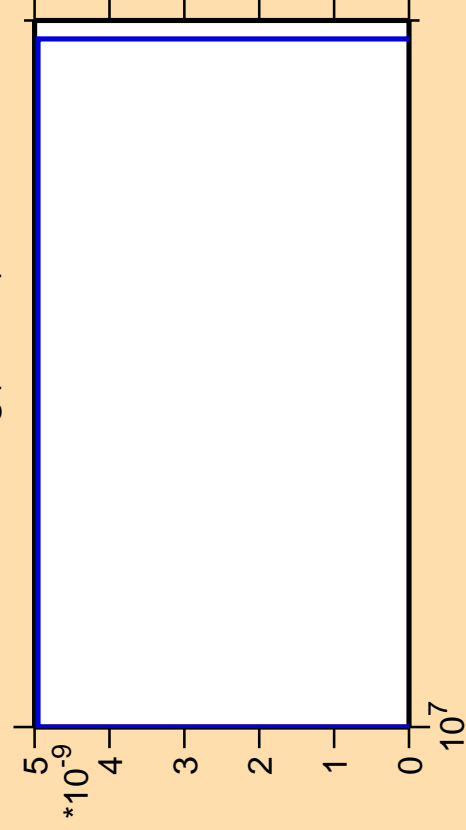
\Delta\sigma/\sigma vs. E for ^{183}\text{Hg} (mt 11)
