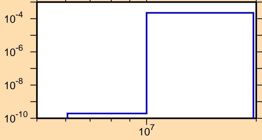
\sigma vs. E for ^{183}\text{Hg}(n,t)
