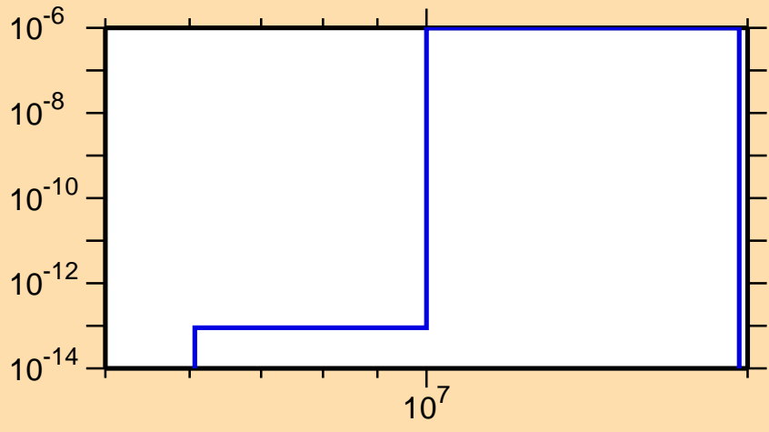
\sigma vs. E for ^{183}\text{Hg}(n,\text{pd})
