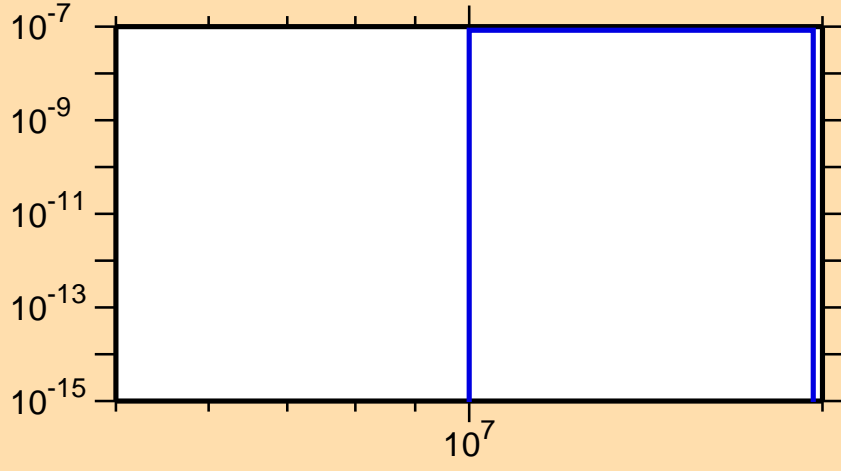
\sigma vs. E for ^{183}\text{Hg}(n,\text{pt})
