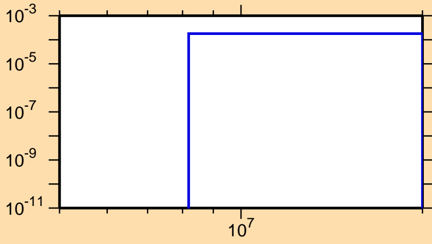
\sigma vs. E for ^{183}\text{Hg}(n,t)
