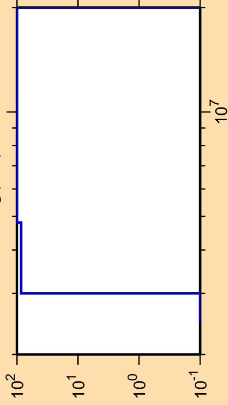
\Delta\sigma/\sigma vs. E for ^{183}\text{Hg}(n,d)
