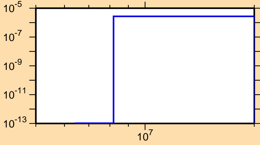
\sigma vs. E for ^{183}\text{Hg} (mt 45)
