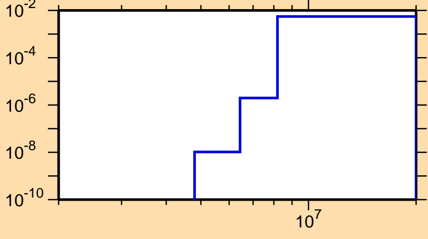
\sigma vs. E for ^{183}\text{Hg}(n,d)
