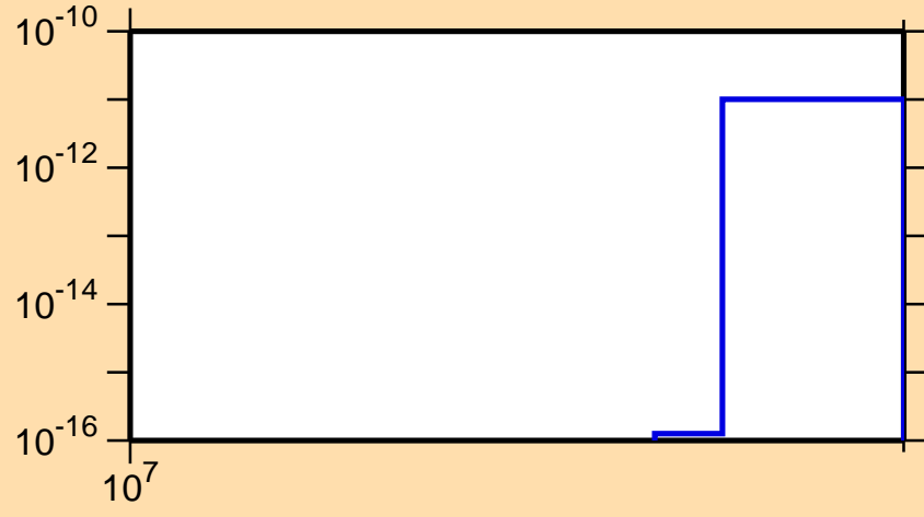
\sigma vs. E for ^{184}\text{Hg}(n,nt)
