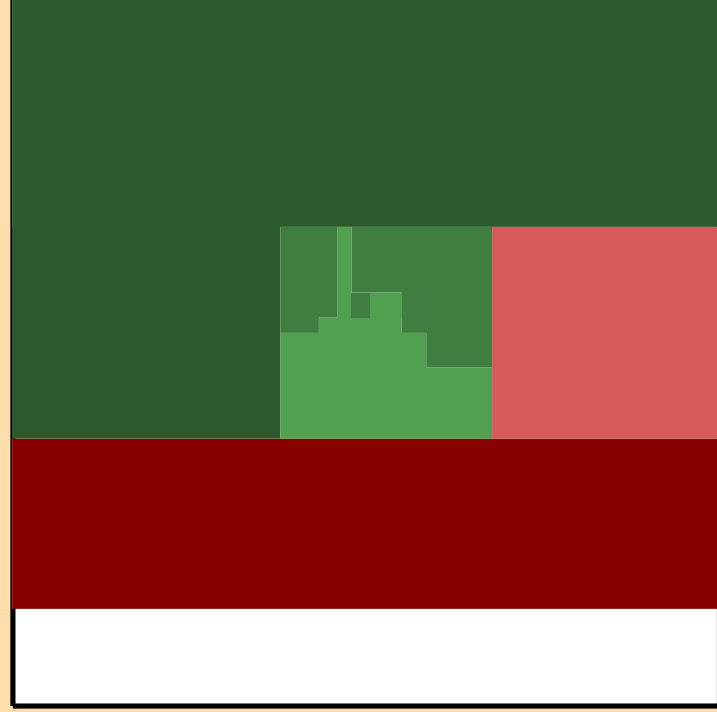
\Delta\sigma/\sigma vs. E for ^{184}\text{Hg}(n,\text{el.})
