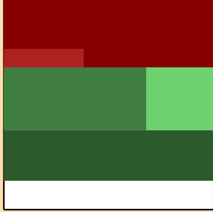
\Delta\sigma/\sigma vs. E for ^{184}\text{Hg}(n,\text{nonel.})
