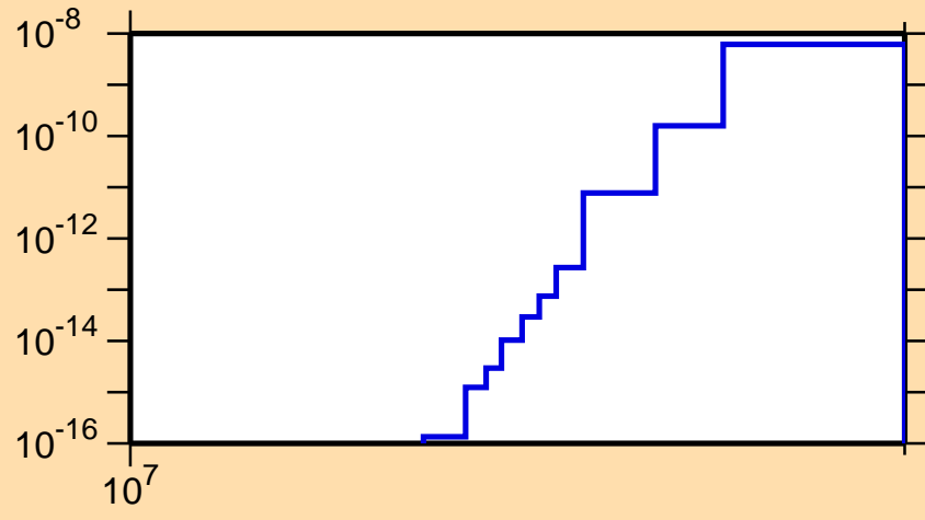
\sigma vs. E for ^{184}\text{Hg}(n,\text{pt})
