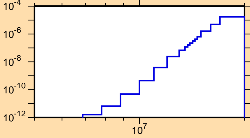
\sigma vs. E for ^{184}\text{Hg}(n,\text{He}3)
