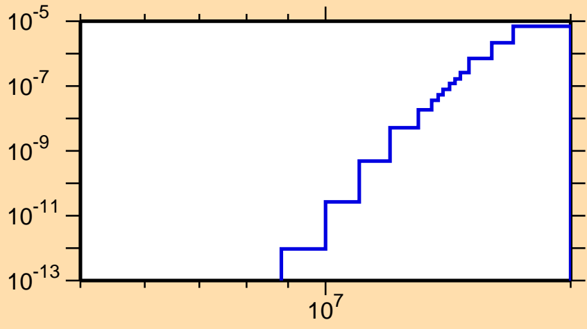
\sigma vs. E for ^{184}\text{Hg} (mt 45)
