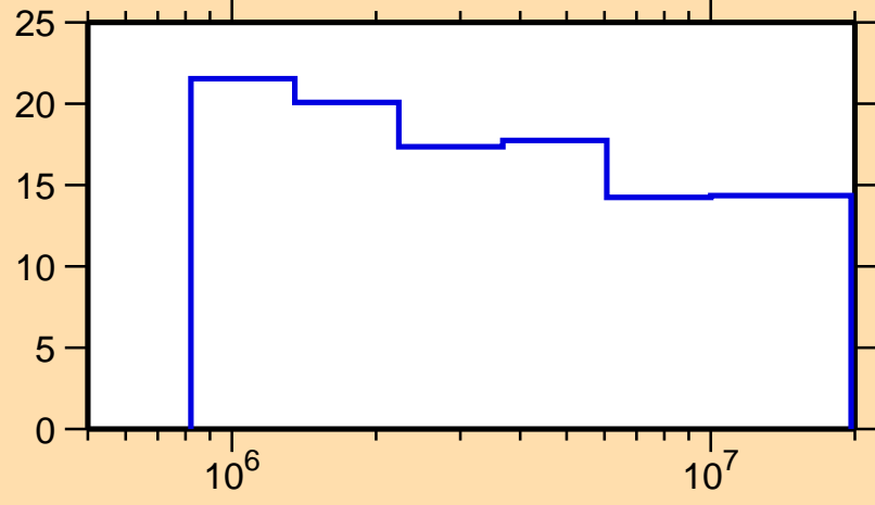
\Delta\sigma/\sigma vs. E for ^{184}\text{Hg}(n,el.)
