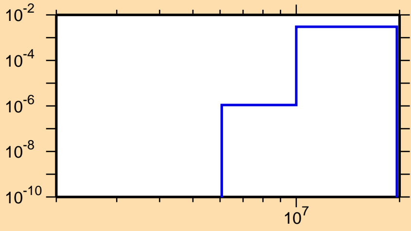
\sigma vs. E for ^{184}\text{Hg}(n,d)
