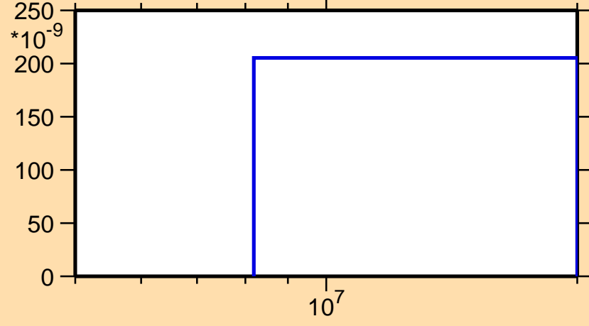
\sigma vs. E for ^{184}\text{Hg}(n,2np)
