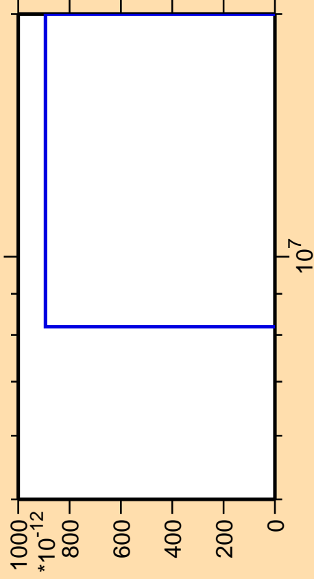
\Delta\sigma/\sigma vs. E for ^{184}\text{Hg} (mt 11)
