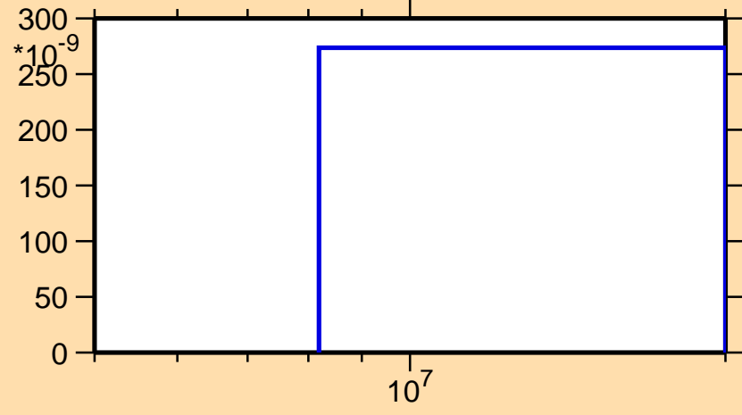
\sigma vs. E for ^{184}\text{Hg} (mt 45)
