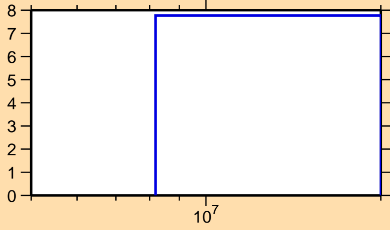
\Delta\sigma/\sigma vs. E for ^{184}\text{Hg}(n,\text{nonel.})
