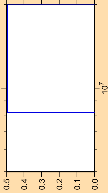
\Delta\sigma/\sigma vs. E for ^{184}\text{Hg}(n,\text{nt})
