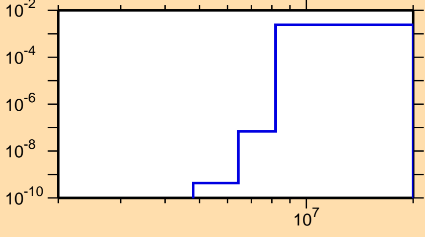
\sigma vs. E for ^{184}\text{Hg}(n,d)
