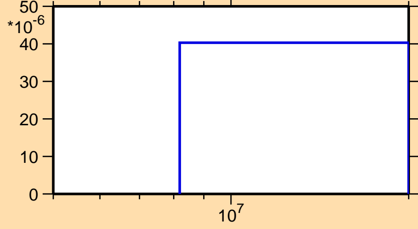
\sigma vs. E for ^{184}\text{Hg}(n,t)
