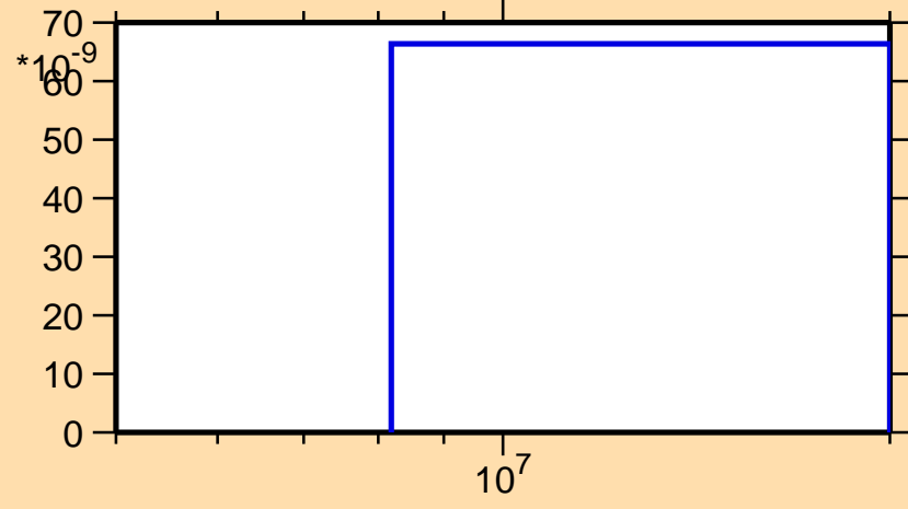
\sigma vs. E for ^{184}\text{Hg}(n,\text{pd})
