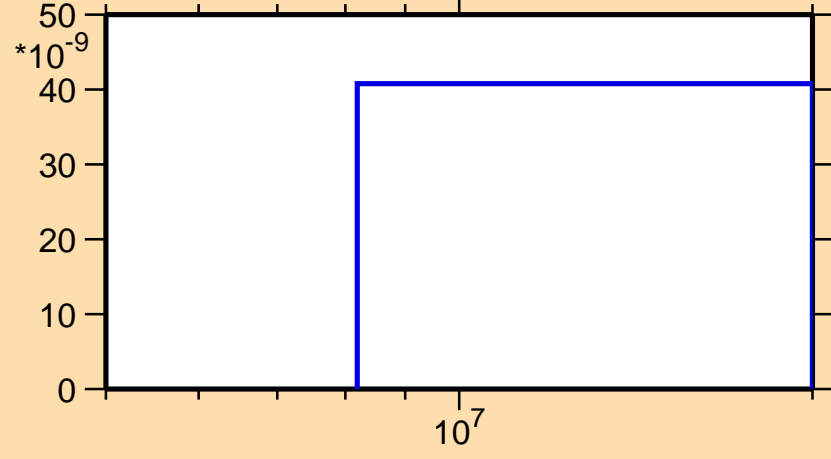
\sigma vs. E for ^{184}\text{Hg}(n,3n)
