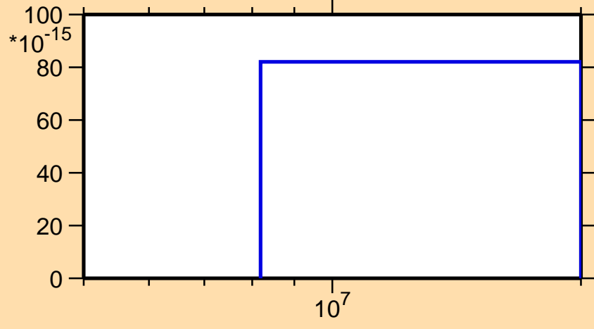
\sigma vs. E for ^{184}\text{Hg}(n,\text{nt})
