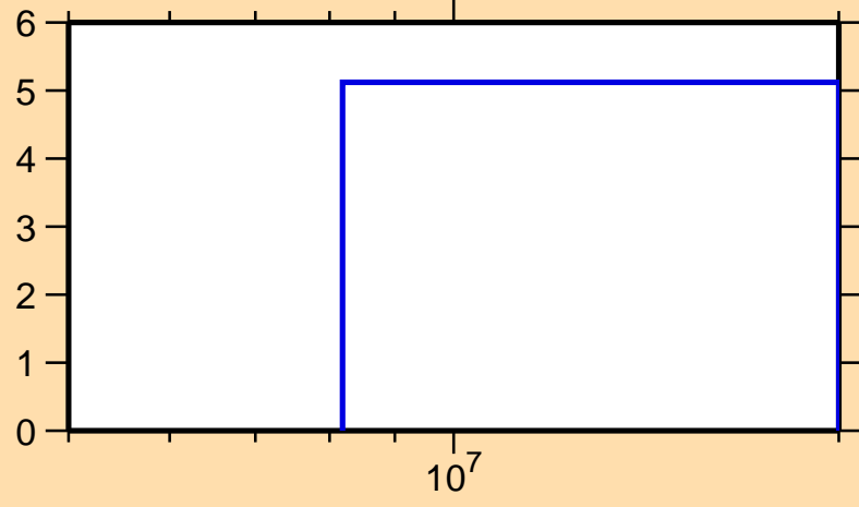
\Delta\sigma/\sigma vs. E for ^{184}\text{Hg}(n,\text{tot.})
