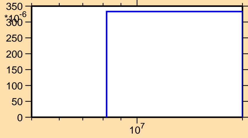
\sigma vs. E for ^{184}\text{Hg}(n,2n\alpha)
