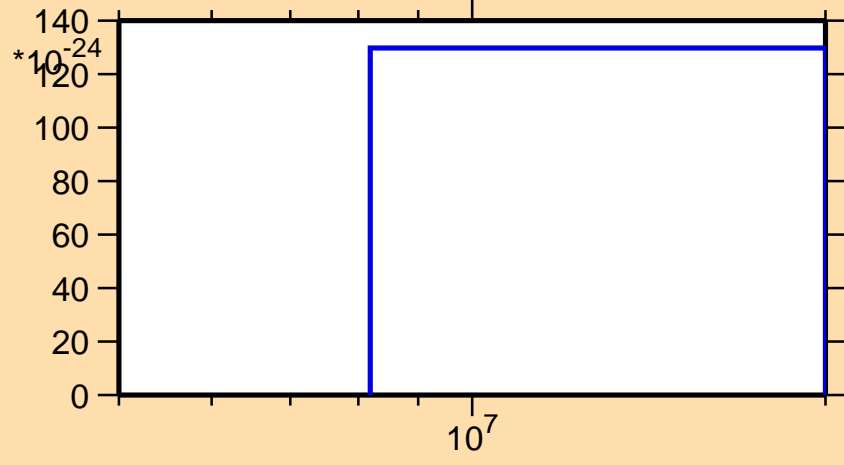
\sigma vs. E for ^{184}\text{Hg} (mt 11)
