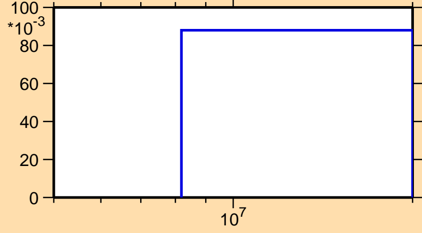
\sigma vs. E for ^{184}\text{Hg}(n,2n)
