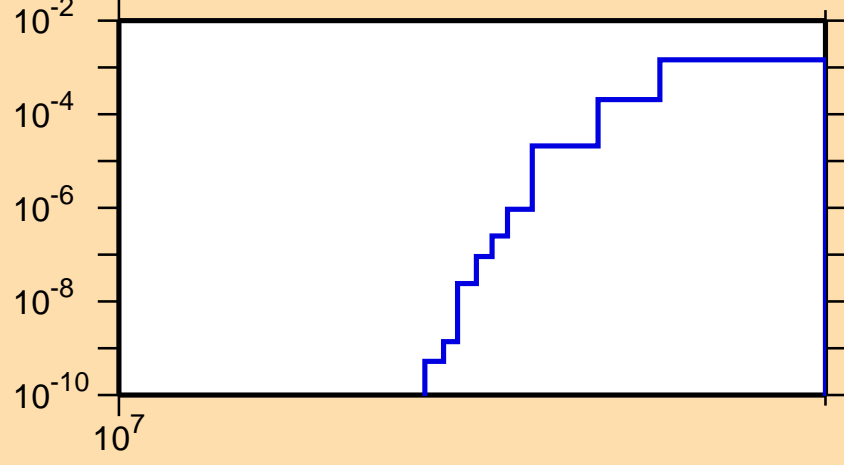
\sigma vs. E for ^{185}\text{Hg}(n,2np)
