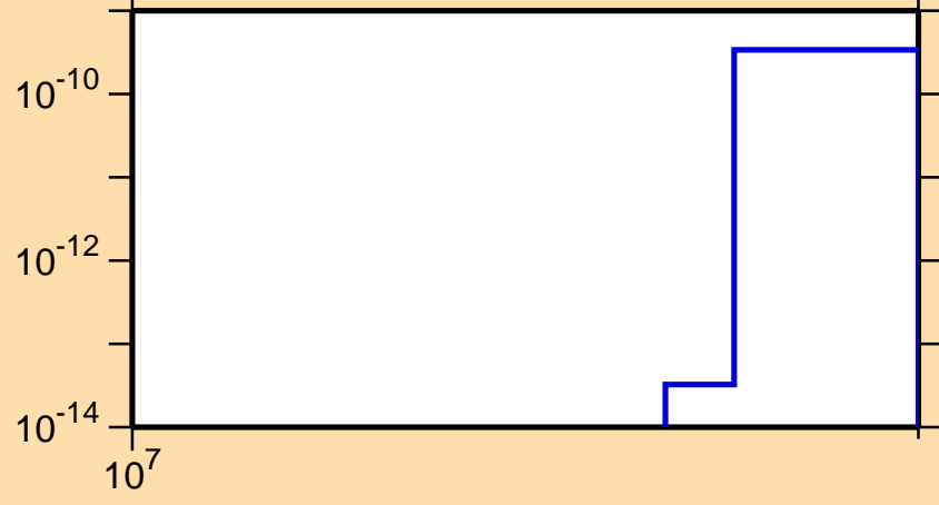
\sigma vs. E for ^{185}\text{Hg}(n,nt)
