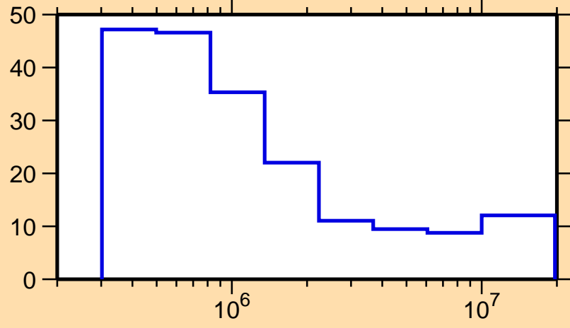
\Delta\sigma/\sigma vs. E for ^{185}\text{Hg}(n,n\text{onel.})
