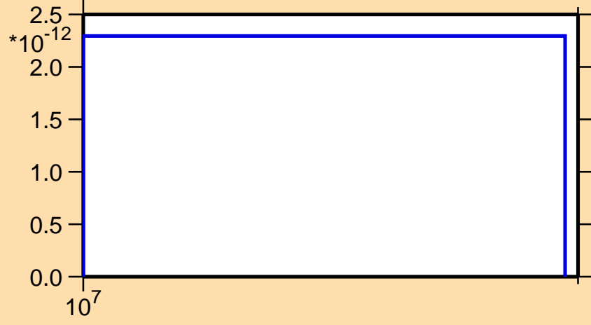
\sigma vs. E for ^{185}\text{Hg}(n,\text{nt})
