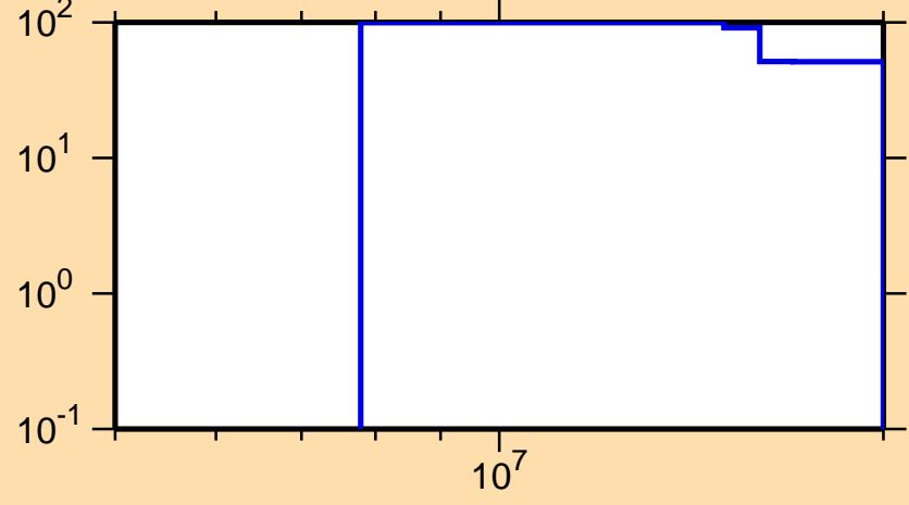
\Delta\sigma/\sigma vs. E for ^{185}\text{Hg}(n,2n)
