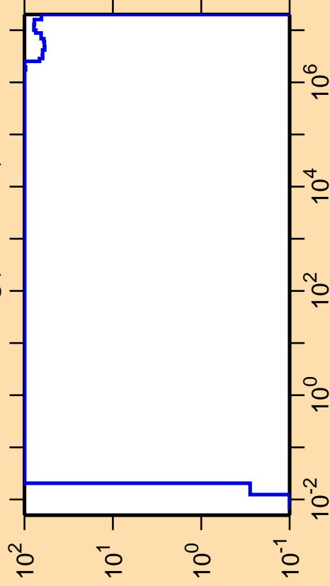
\Delta\sigma/\sigma vs. E for ^{185}\text{Hg}(n,\text{ncont.})
