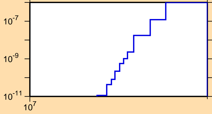
\sigma vs. E for ^{185}\text{Hg}(n,\text{nd})
