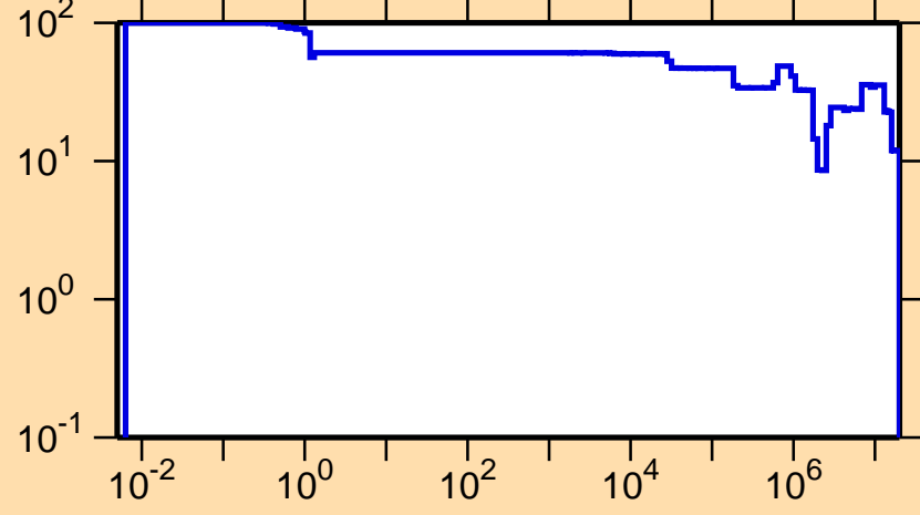
\Delta\sigma/\sigma vs. E for ^{185}\text{Hg}(n,\text{el.})
