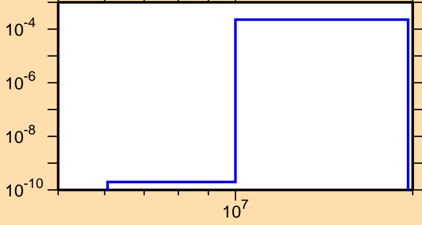
\sigma vs. E for ^{185}\text{Hg}(n,t)
