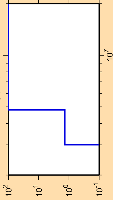
\Delta\sigma/\sigma vs. E for ^{185}\text{Hg}(n,d)
