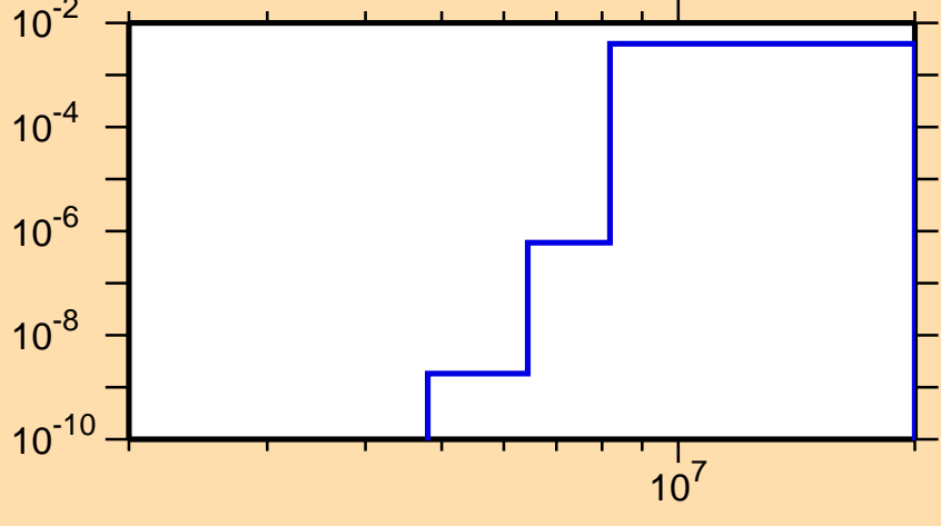
\sigma vs. E for ^{185}\text{Hg}(n,d)
