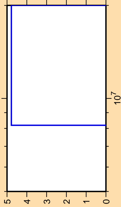
\Delta\sigma/\sigma vs. E for ^{185}\text{Hg}(n,\text{nt})
