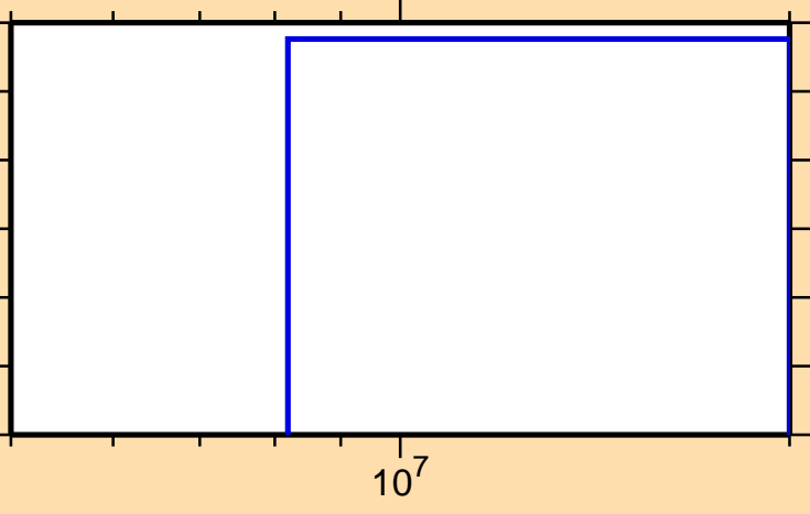
\sigma vs. E for ^{185}\text{Hg}(n,\text{nt})
