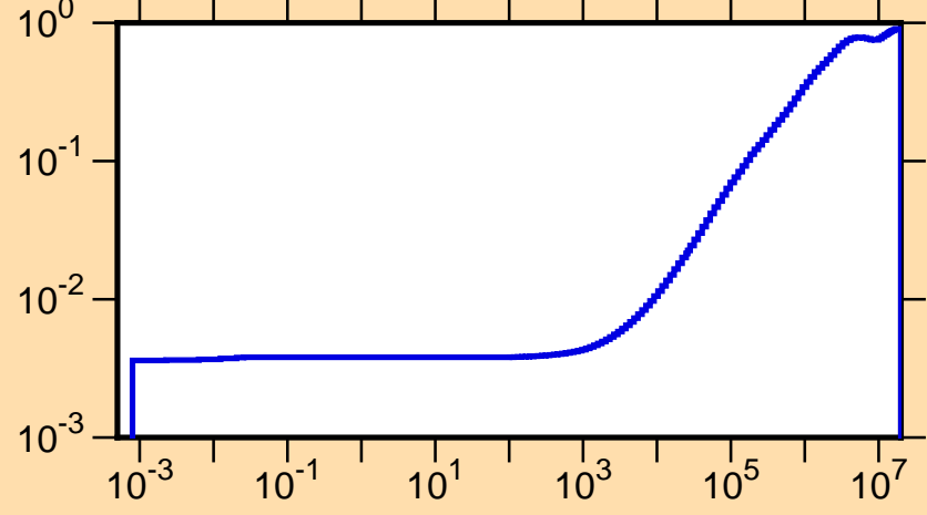
\mu vs. E for ^{187}\text{Hg}(\text{mt251})
