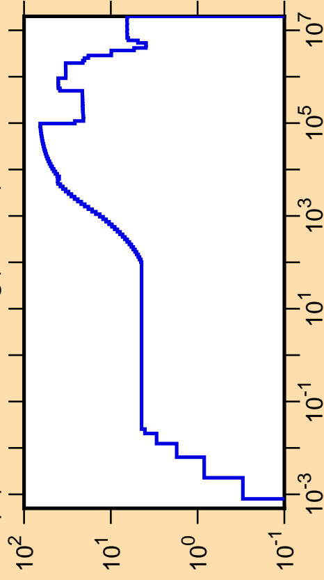
\Delta\mu/\mu vs. E for ^{187}\text{Hg}(\text{mt251})
