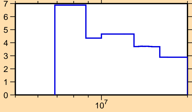
\Delta\sigma/\sigma vs. E for ^{187}\text{Hg}(n,\text{tot.})
