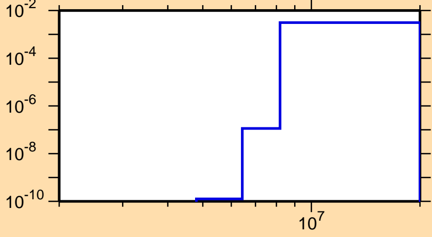
\sigma vs. E for ^{187}\text{Hg}(n,d)
