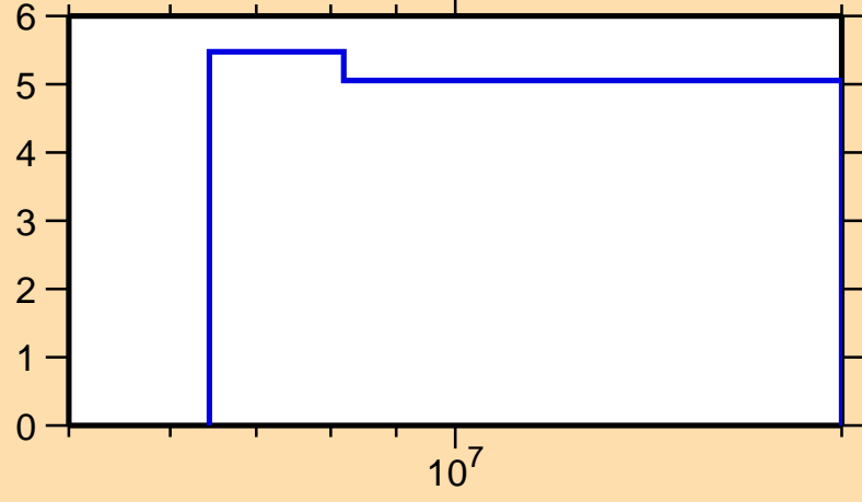
\Delta\sigma/\sigma vs. E for ^{187}\text{Hg}(n,\text{nonel.})
