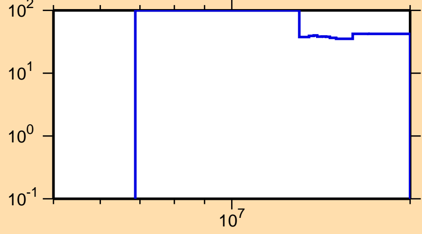
\Delta\sigma/\sigma vs. E for ^{187}\text{Hg}(n,2n)
