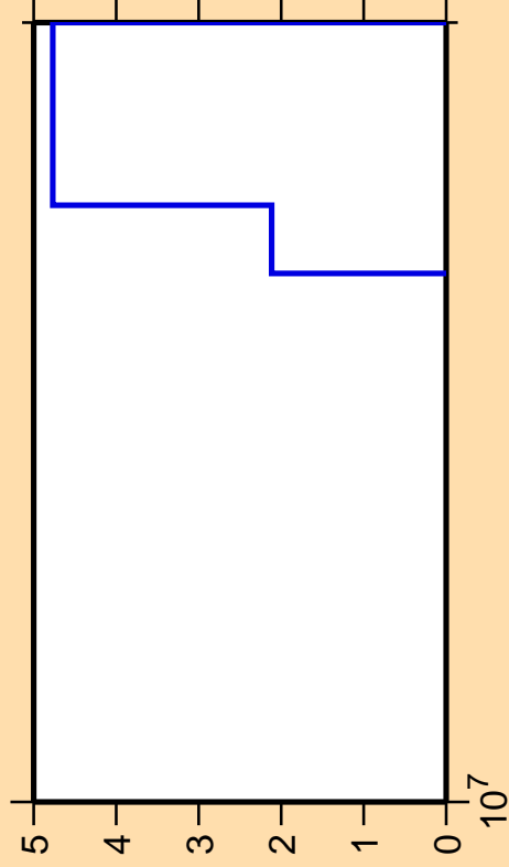
\Delta\sigma/\sigma vs. E for ^{187}\text{Hg}(n,3n\alpha)
