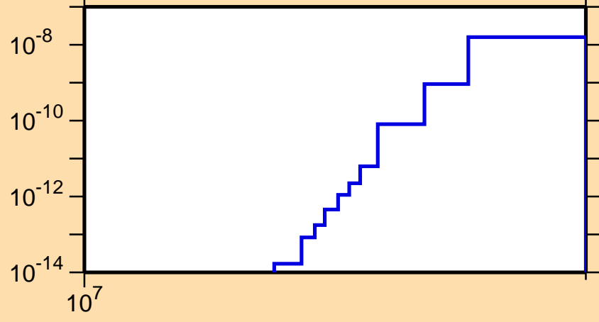
\sigma vs. E for ^{187}\text{Hg}(n,\text{pt})
