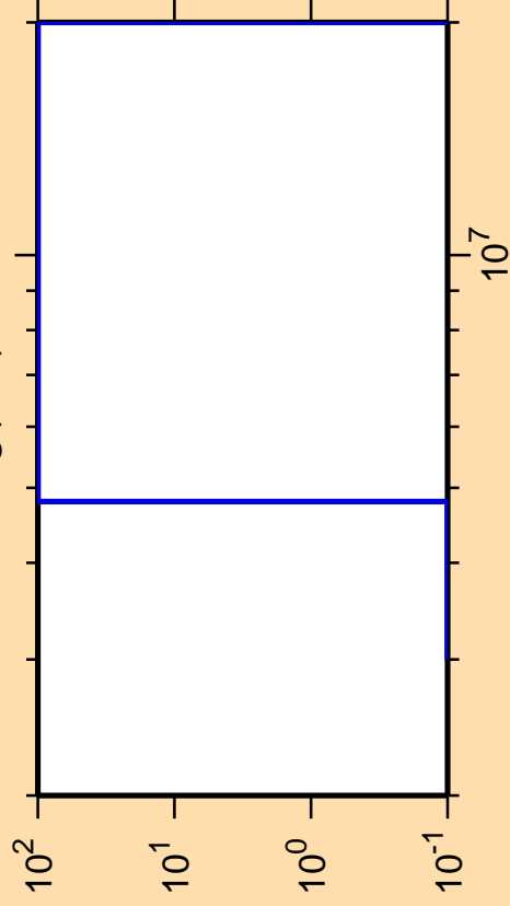
\Delta\sigma/\sigma vs. E for ^{187}\text{Hg}(n,d)
