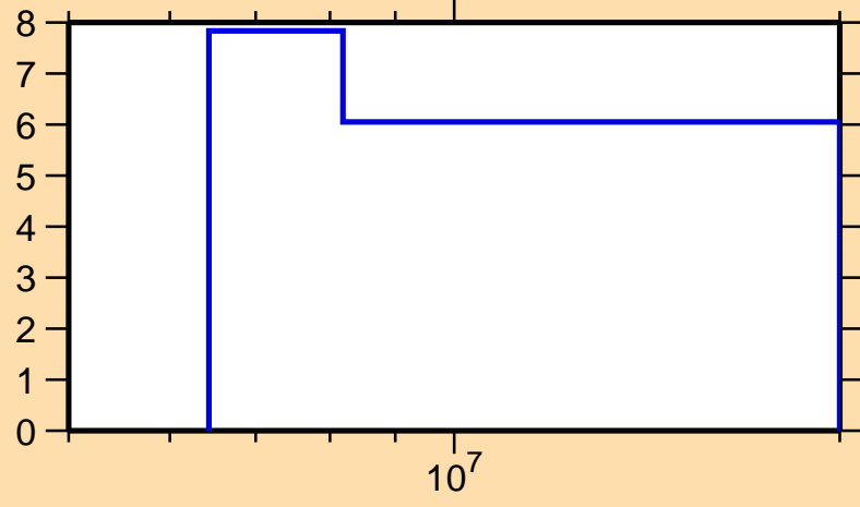
\Delta\sigma/\sigma vs. E for ^{187}\text{Hg}(n,\text{nonel.})
