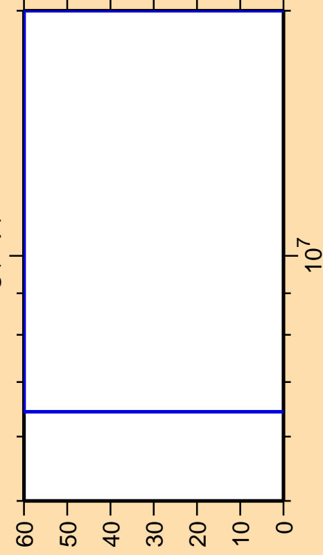
\Delta\sigma/\sigma vs. E for ^{187}\text{Hg}(n,p)
