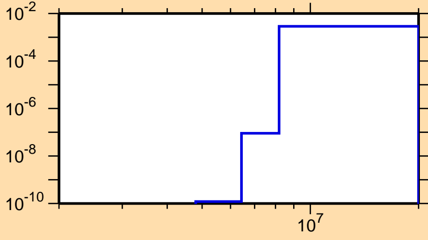
\sigma vs. E for ^{187}\text{Hg}(n,d)
