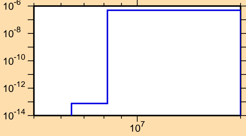
\sigma vs. E for ^{187}\text{Hg}(n,\text{He3})
