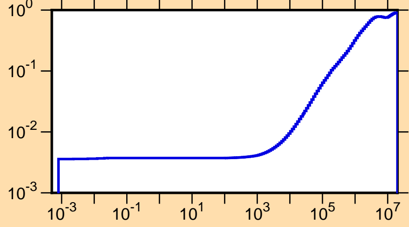
\mu vs. E for ^{188}\text{Hg}(\text{mt251})
