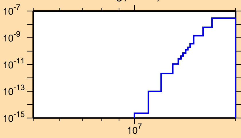
\sigma vs. E for ^{188}\text{Hg} (mt 45)
