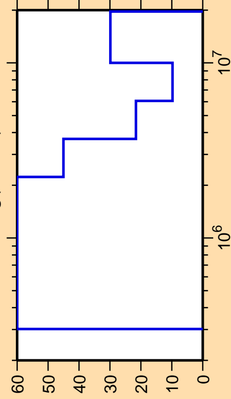
\Delta\sigma/\sigma vs. E for ^{188}\text{Hg}(n,\text{inel.})
