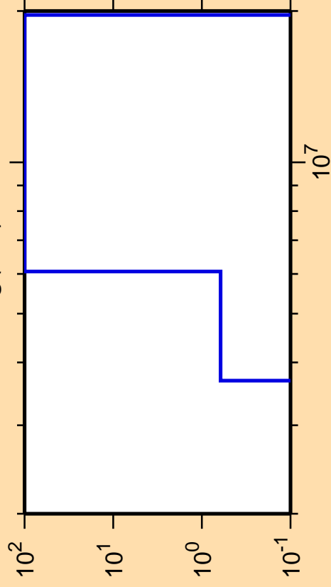
\Delta\sigma/\sigma vs. E for ^{188}\text{Hg}(n,d)
