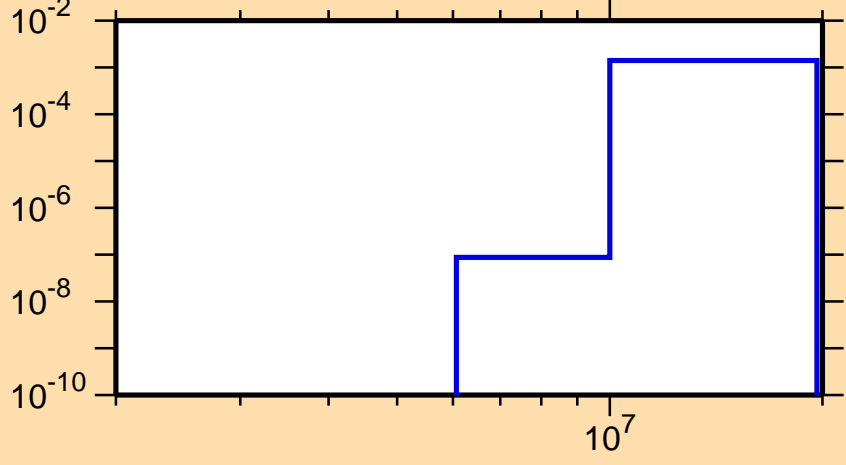
\sigma vs. E for ^{188}\text{Hg}(n,d)
