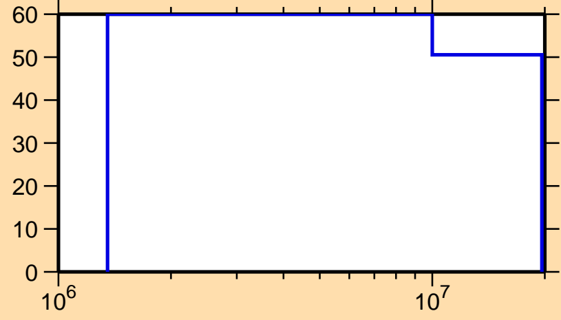
\Delta\sigma/\sigma vs. E for ^{188}\text{Hg}(n,n_1)
