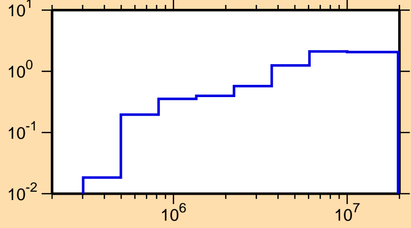
\sigma vs. E for ^{188}\text{Hg}(n,\text{inel.})
